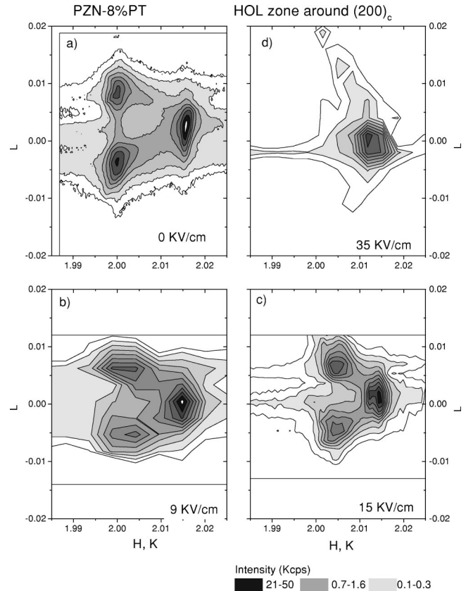
FIG. 5. Mesh scans around the pseudocubic (200) reflection in the HOL (or OKL ) zone of reciprocal space for 8PT at E=0 (a), 9 (b), 15 (c), and 35 (d) kV/cm. The intensities are plotted on a logarithmic scale.
