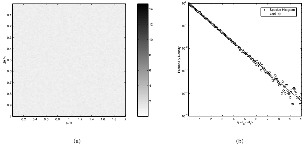
Fig. 2. (a) Speckle pattern formed by the angular-resolved backscattering light. (b) Normalized speckle I_x/\langle I_x \rangle follows a negative exponential distribution.
