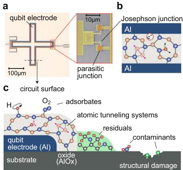
Fig. 1 Overview of defect types in superconducting qubits. a Photograph of the cross-shaped capacitor electrode of a transmon qubit that is connected to the ground plane via Josephson junctions. 22 Inset: The small junctions are contacted via large-area parasitic junctions (shaded orange). b Illustration of defect types in the amorphous \text{AlO}_x tunnel barrier of a Josephson junction, indicating atomic tunnelling systems, hydrogen impurities, and trapped electrons. c Sketch of surface defects, showing a cross-section of the qubit electrode and its native aluminium oxide which hosts structural TLS (not to scale). In addition, adsorbates such as hydrogen (H) and molecular oxygen ( \text{O}_2 ) provide surface spins. Fabrication residuals such as photoresist, atmospheric contaminants, and substrate surface amorphization due to circuit patterning are further sources of surface defects.
