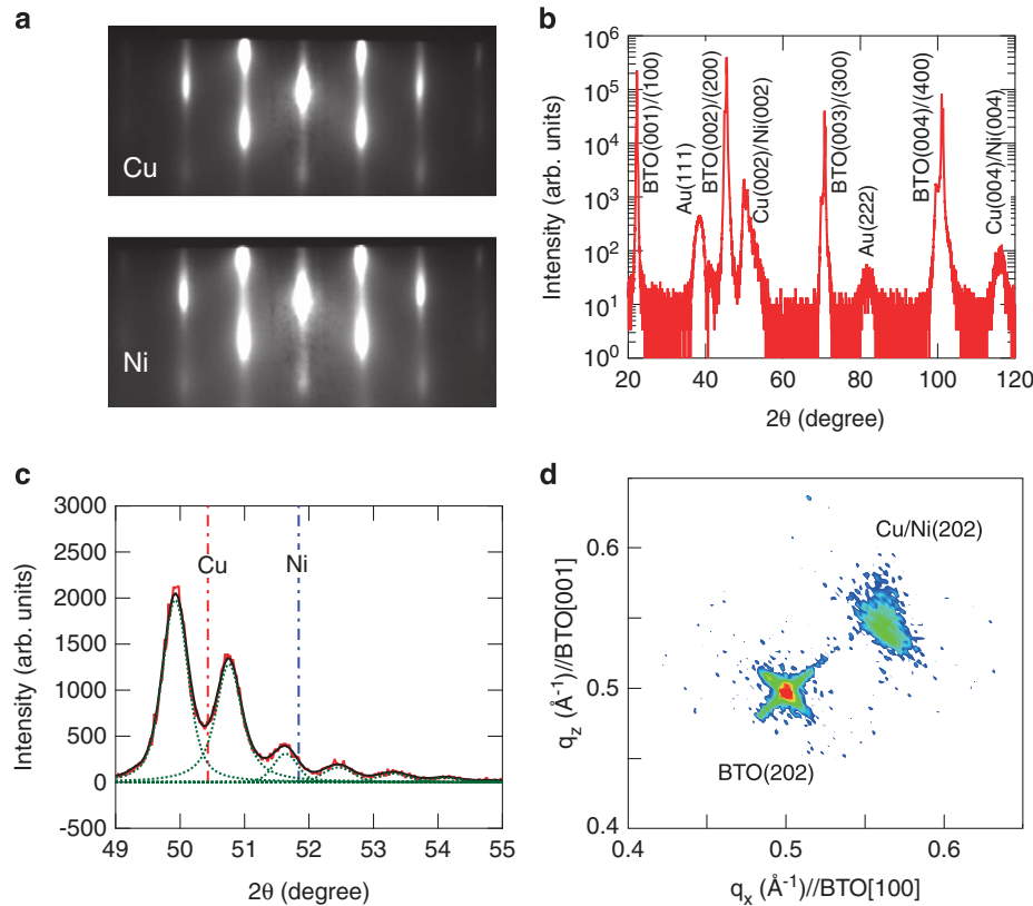
Figure 1 (a) RHEED images of the top Ni and Cu layers along the \langle 100 \rangle direction of BaTiO 3 . (b) X-ray diffraction spectrum of a [Cu(9 nm)/Ni(2 nm)] 5 /Cu(9 nm)/Fe(1 nm)/BaTiO 3 (001) heterostructure and (c) an expanded view of an interference fringe from the Cu/Ni multilayer. The black solid curve in c is a fit to the experimental data using Voigt functions (green dotted lines) to match the satellite peaks. The red and blue dash-dotted lines indicate the diffraction angles of bulk Cu(002) and Ni(002). (d) Reciprocal lattice map around the (202) diffraction peaks of the Cu/Ni multilayer and BaTiO 3 substrate.
