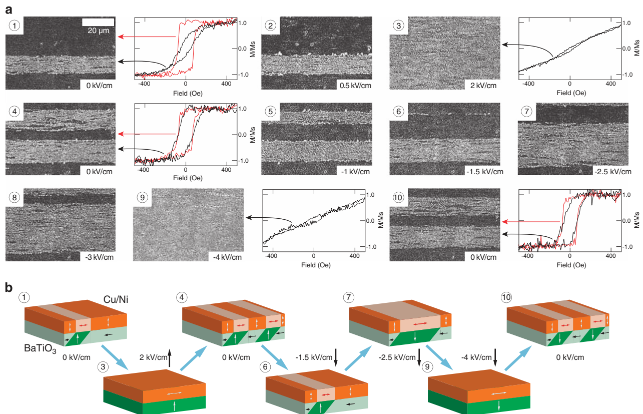
Figure 3 (a) MOKE microscopy images (measured in zero magnetic field) and local polar MOKE curves of the Cu/Ni multilayer as a function of out-of-plane electric field. (b) Schematic illustration of the ferroelectric domain structure in the BaTiO 3 substrate (green) and the magnetic domains of the Cu/Ni multilayer (orange) during the electric-field-controlled switching sequence in a.
