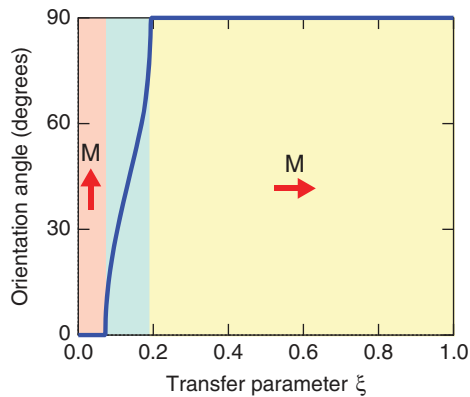
Figure 4 Calculated orientation of the equilibrium magnetization direction in the Cu/Ni multilayer after a - to c -domain switching in BaTiO 3 . The parameter \xi indicates the efficiency of strain transfer from the BaTiO 3 substrate to 2-nm thick Ni layers during polarization switching.
