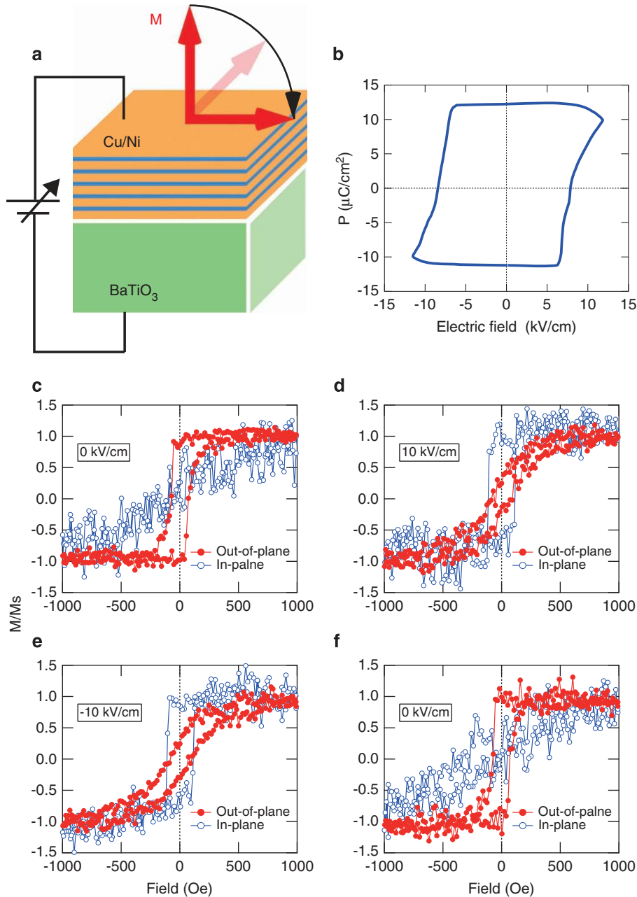
Figure 2 (a) Schematic illustration of the experimental system. (b) Out-of-plane polarization hysteresis curve of the BaTiO 3 substrate. (c–f) Normalized out-of-plane and in-plane magnetic hysteresis curves of the Cu/Ni multilayer recorded while sequentially applying an electric field of (c) E=0\text{ kV cm}^{-1} , (d) E=10\text{ kV cm}^{-1} , (e) E=-10\text{ kV cm}^{-1} and (f) E=0\text{ kV cm}^{-1} across BaTiO 3 .
