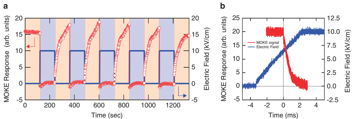
Figure 5 (a) Time-resolved polar MOKE response of the Cu/Ni multilayer on BaTiO 3 during on and off switching of a 10 \text{ kV cm}^{-1} electric field. (b) Zoom-in of the MOKE response during the application of a positive electric-field pulse.
