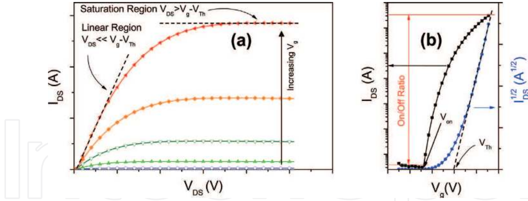
Figure 6. Characteristic curves of TFTs (a) output curves with characteristic linear and saturation regions; (b) transfer curve and I^{1/2} versus v_g (linear scale) extrapolation of V_{th} and slope for saturation mobility determination;
