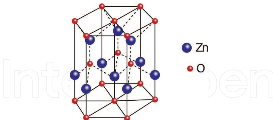
Figure 1. Representation of the ZnO unit cell with wurtzite structure.
