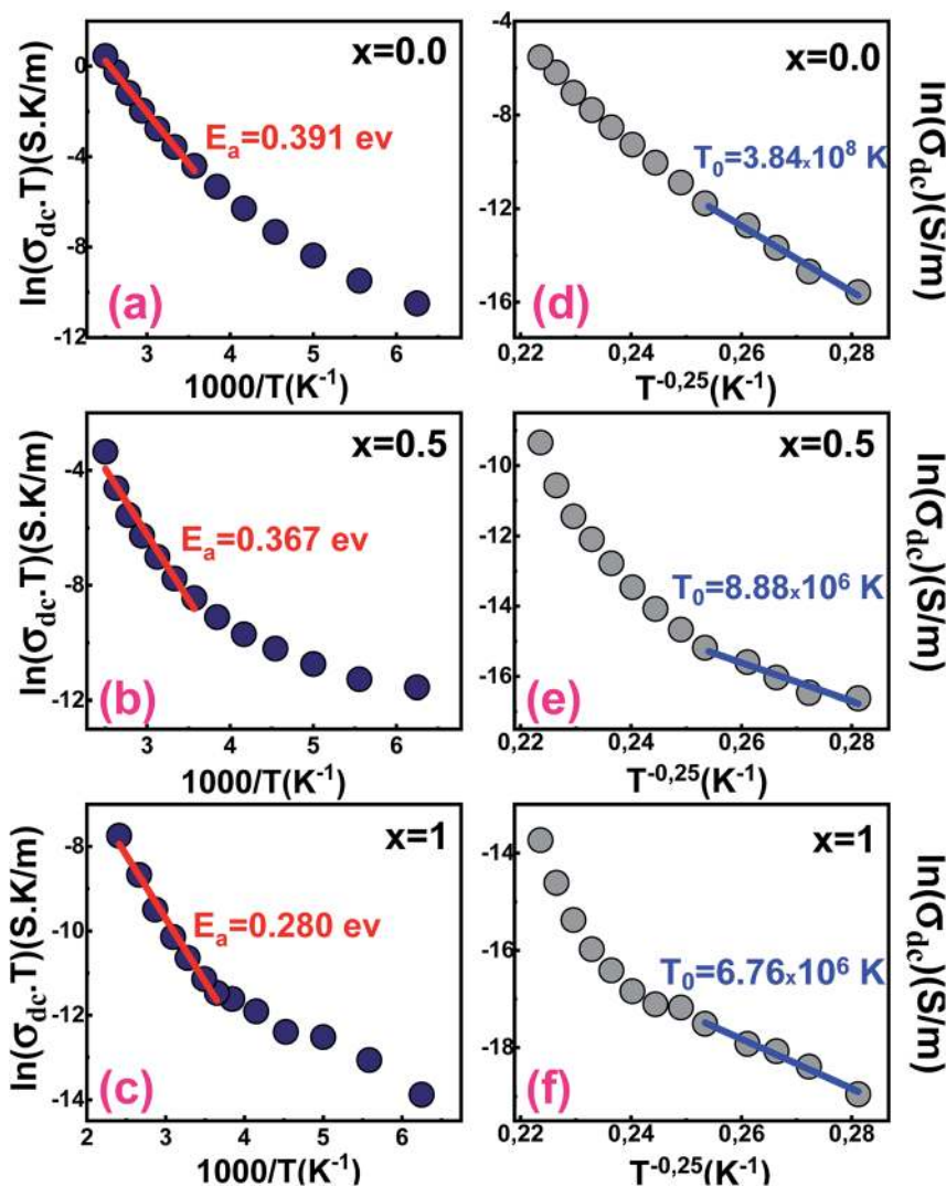
Fig. 6 Variation of \ln(\sigma_{dc}T) vs. (1000/T) of \text{Ba}_{1-x}\text{Sr}_x\text{Fe}_{12}\text{O}_{19} [(a) x = 0.0 , (b) x = 0.5 and (c) x = 1 ]. Variation of \ln(\sigma_{dc}) vs. (T^{-0.25}) of \text{Ba}_{1-x}\text{Sr}_x\text{Fe}_{12}\text{O}_{19} [(d) x = 0.0 , (e) x = 0.5 and (f) x = 1 ].
