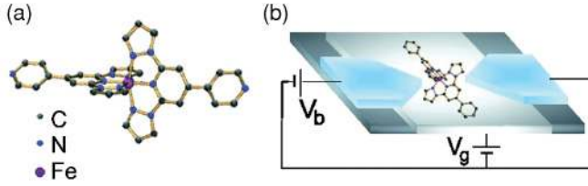
FIG. 5. (Color online) Left: The spin transition complex together with the linker units that were employed in the experimental measurements: [\text{Fe} - (\text{L})_2]^{2+} complex [ \text{L} = 4'-(4'''-\text{pyridyl})-1,2':6'1''\text{-bis-(pyrazolyl)pyridine} ]. Right: Schematic representation of the three-terminal device setup.
