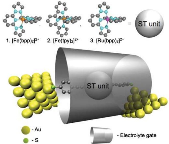
FIG. 2. (Color online) Top: Atomic structure of the complexes 1 ( [Fe(bpp)_2]^{2+} ), bpp—bispyrazolyl pyridine 2 ( [Fe(tpy)_2]^{2+} ), tpy—terpyridine and 3 ( [Ru(bpp)_2]^{2+} ). (The molecular complex used in the experiment has in addition to 1 pyridine anchor groups.) Colors: dark gray: carbon; cyan (light gray): nitrogen; red (gray): iron; magenta (gray): ruthenium; hydrogen atoms are not displayed. Bottom: model geometry of a single molecule transport measurement. 8,13,32–34 The surrounding cylinder models an electrolyte gate.
