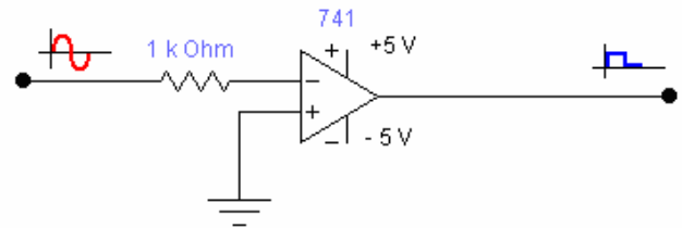
Figure 5. Sampling Circuit.
