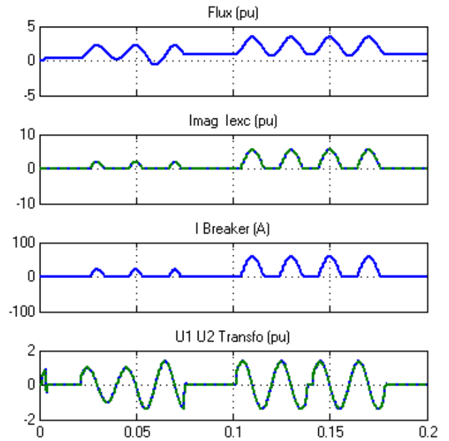
Figure 22. TR1 transformer electrical parameters of the change.
