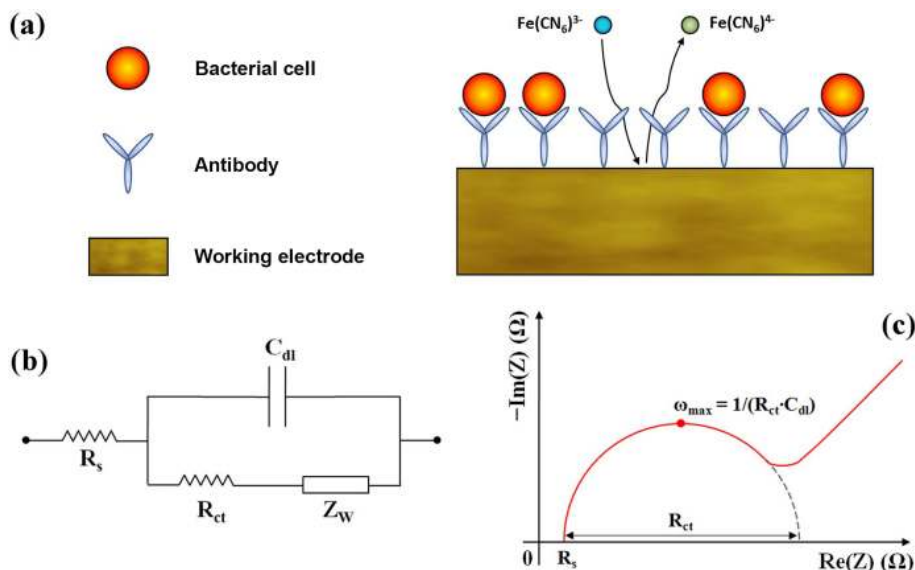
Figure 3. (a) Modified working electrode with immobilized bioreceptor; (b) equivalent electrical circuit of the biosensor; (c) Nyquist plot of the equivalent circuit.
