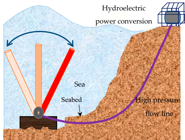
Figure 6. Floating device of oscillating wave surge converter.
