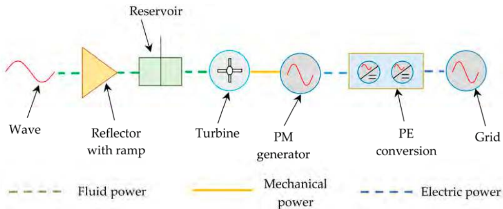
Figure 17. Electrical harnessing equipment from OWE using Wave Dragon.
