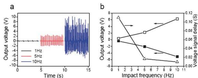
Fig. 3 a) Voltage outputs of a nanofibre device under different impact frequencies. b) Dependences of output voltages and delay time of the opposite voltage on impact frequency. □: positive voltage outputs, ■: negative voltage outputs, △: voltage signal delay. Membrane thickness = 140 \mu\text{m} ; working area = 2 \text{cm}^2 .
