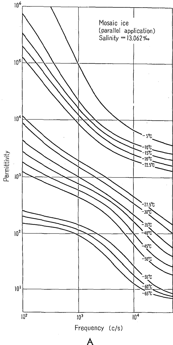
Fig. 3. Dispersions of the permittivity (Fig. 3A) and the conductivity (Fig. 3B) of the mosaic ice. Brine cells are arranged parallel to the applied electric field
