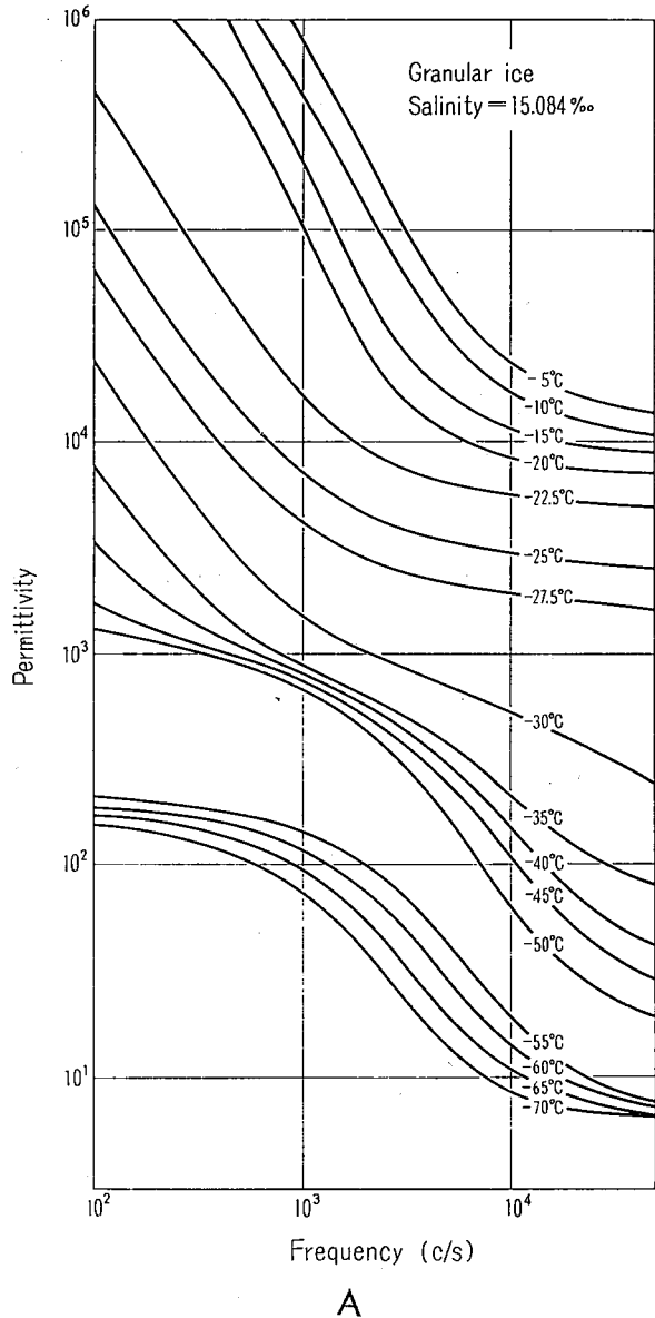
Fig. 4. Dispersions of the permittivity (Fig. 4A) and the conductivity (Fig. 4B) of the granular ice
