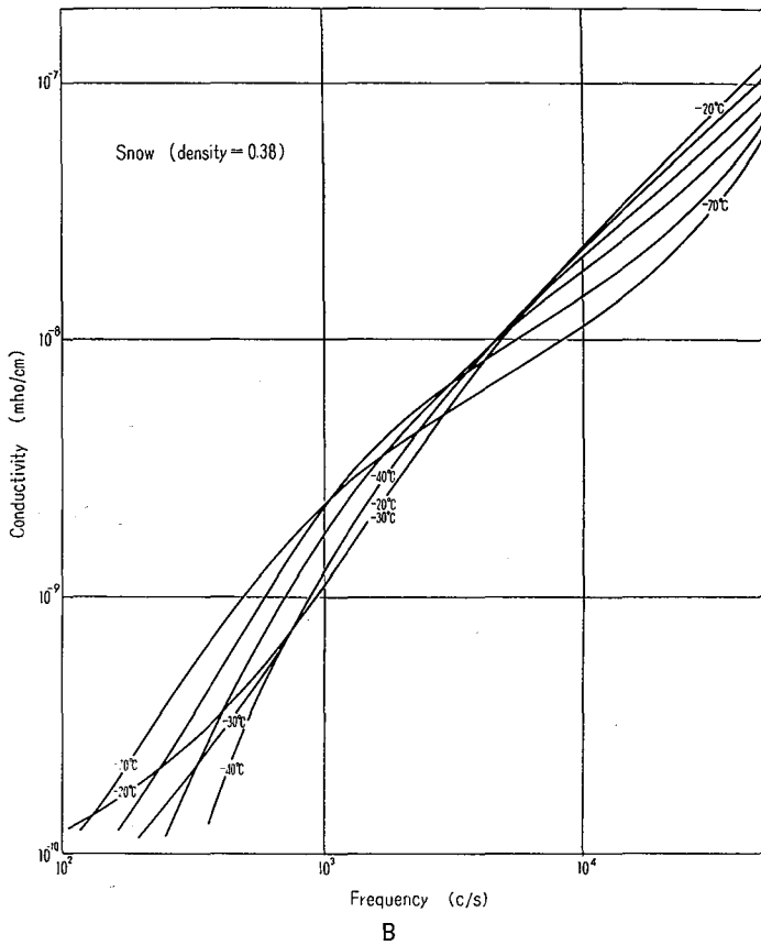
Fig. 6. Dispersions of the permittivity (Fig. 6 A) and the conductivity (Fig. 6 B) of snow
