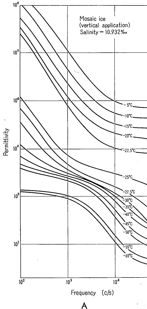
Fig. 2. Dispersions of the permittivity (Fig. 2A) and the conductivity (Fig. 2B) of the mosaic ice. Brine cells are arranged vertical to the applied electric field
