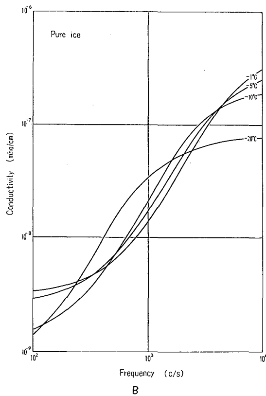
Fig. 5. Dispersions of the permittivity (Fig. 5A) and the conductivity (Fig. 5B) of pure ice
