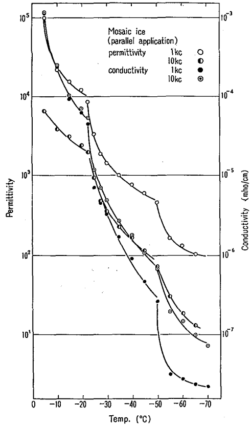
Fig. 8. Temperature dependence of the permittivity and the conductivity of the mosaic ice. The field is applied in parallel
