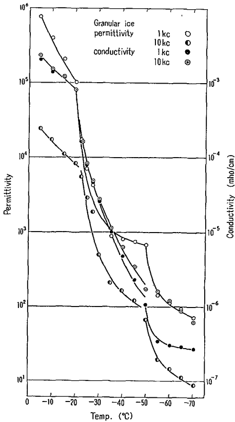
Fig. 9. Temperature dependence of the permittivity and the conductivity of the granular ice
