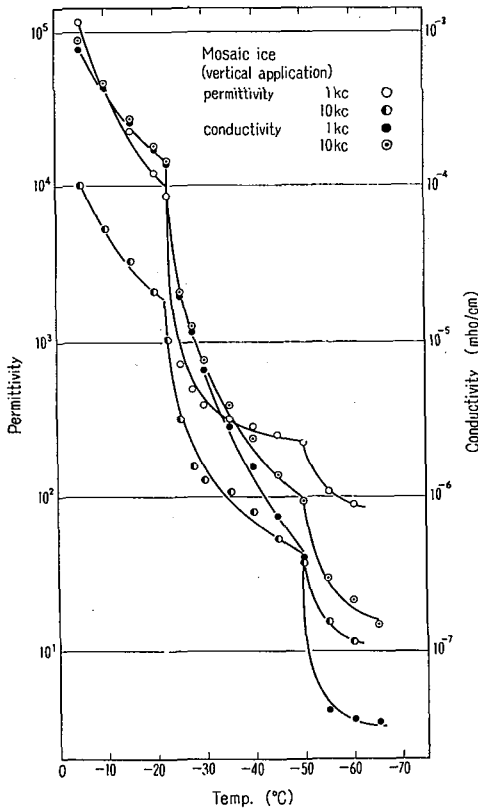
Fig. 7. Temperature dependence of the permittivity and the conductivity of the mosaic ice. The field is applied vertically
