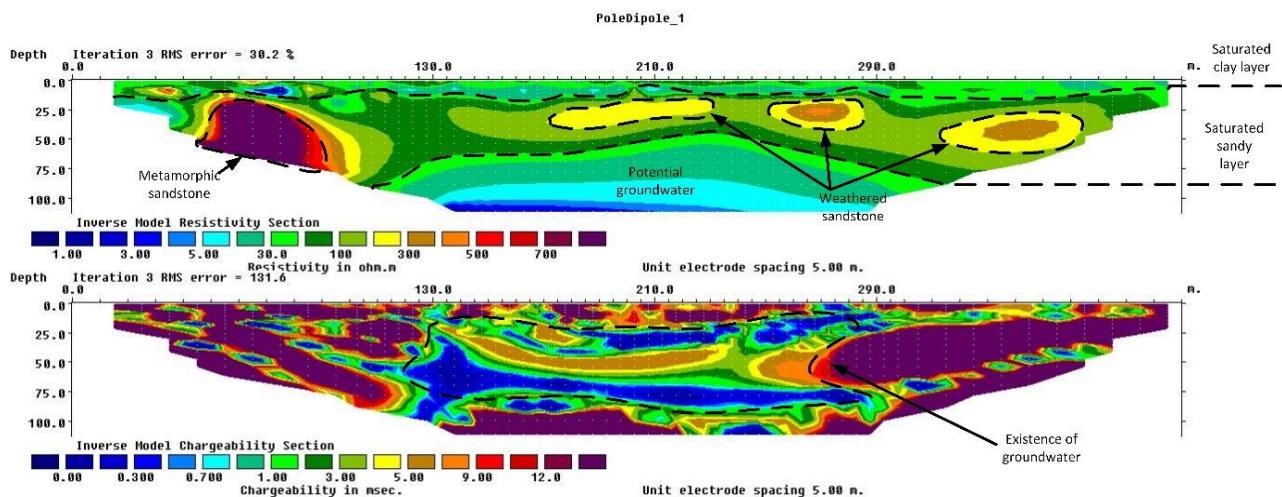
Fig. 6 Resistivity and induced polarization results at Kampung Paya Rawa.
