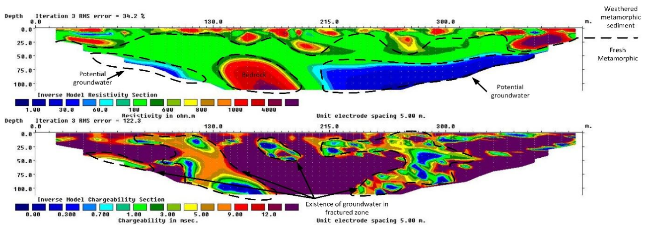
Fig. 5 Resistivity and induced polarization results at Kampung Jongkok Batu.
