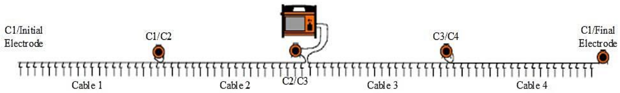
Fig. 4 The arrangement of ABEM Terrameter LS2 resistivity meter and other equipments.
