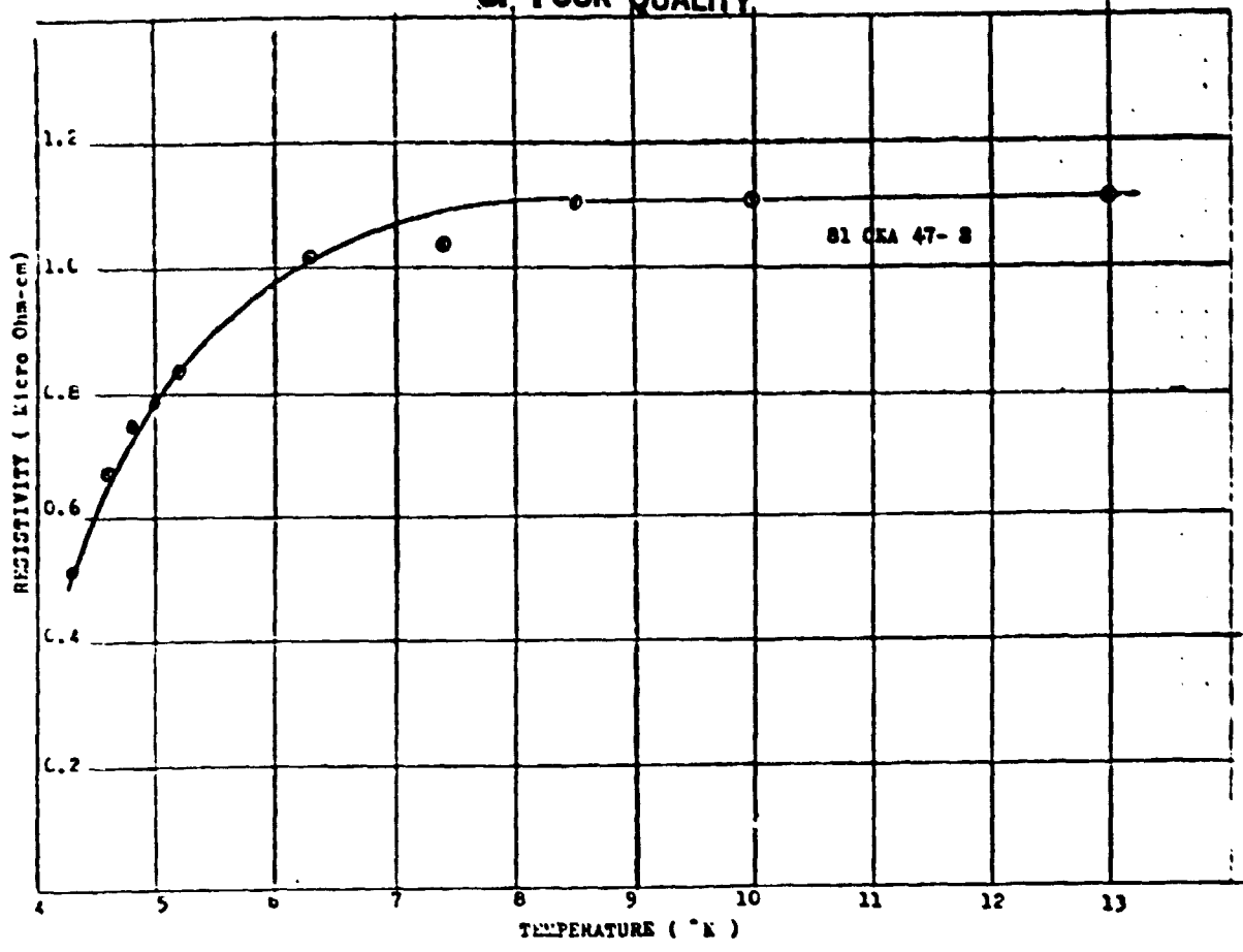
FIGURE 7. Electrical resistivity as a function of temperature for specimen 81CNA47-S at current density of 8.8 A/cm 2 .
