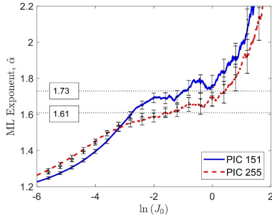
Figure 3. (color online) Maximum-likelihood (ML) fit of PIC 151 (blue solid) and PIC 255 (red dashed). PIC 151 displays a plateau of two decades at -2.0 \leq \ln(J_0) \leq 0.0 with an average estimated exponent \hat{\epsilon} of 1.73. PIC 255 shows a plateau of three decades at -3.0 \leq \ln(J_0) \leq 0.0 with \hat{\epsilon} of 1.61. Both averaged exponents have a standard deviation \sigma of \pm 0.04 . The lack of definitive kinks at J_0 = J_{\min} for both ML curves was due to lower cut-off effects that arose from saturation effects in the measurement apparatus [38].
