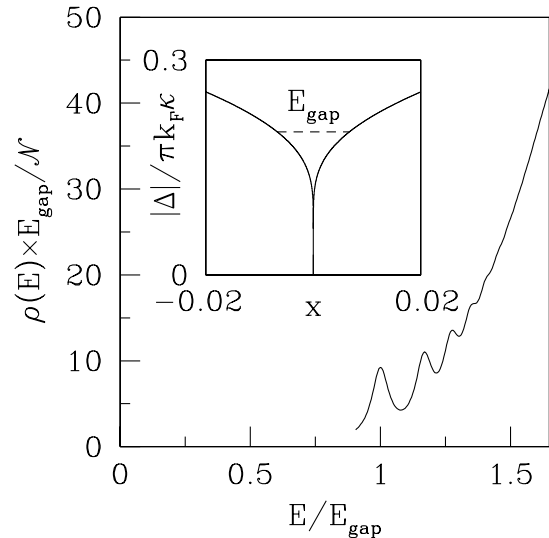
FIG. 2. Low-energy density of states \rho(E) of the effective Hamiltonian (10), related to \rho(\omega) of the biharmonic Eq. (14) by Eq. (18). The plot is for |\ln\epsilon| = 10 and has been smoothed with a Lorentzian. The inset shows the logarithmic pair potential appearing in \mathcal{H}_{\text{eff}} , the ground state of which is the excitation gap (dashed line).
