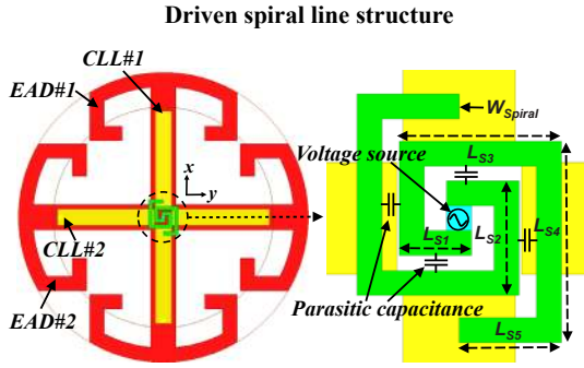
Fig. 1. The spiral line-based HCP antenna. (Left) Bottom view of the antenna and (Right) enlarged view of the driven spiral line element.
