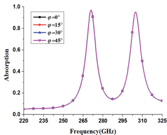
Fig. 7 Absorption spectra for different polarization angles under the normal incident wave. The electric field is changed by an angle \phi with respect to x -direction.
