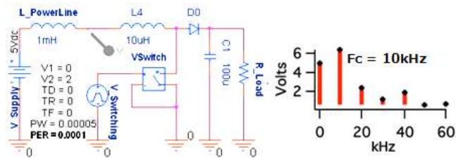
Figure 1: (Left) Circuit model of a SMPS with placement of the voltage probe. (Right) Frequency domain analysis at the voltage probe showing EMI at 10 kHz.
