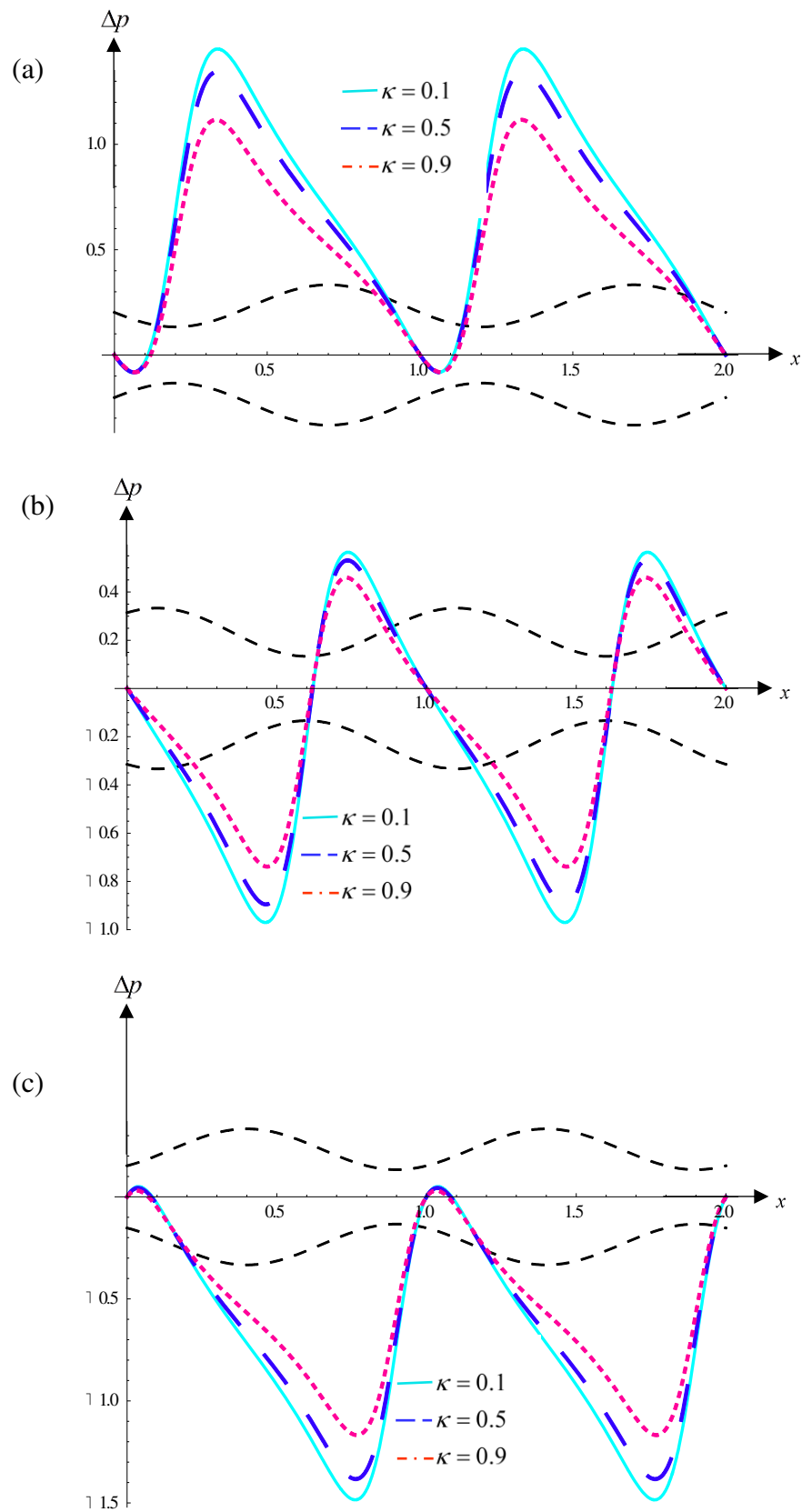
Fig.3. Pressure distribution along the length of tube at \phi=0.6, l=2, U_{HS}=1, \lambda_1=1 at different time period (a) t=0.2 (b) t=0.6 (c) t=0.9 . Color lines represent the pressure distribution for different values of Debye length and Black dotted lines show the train wave propagation and single wave propagation.
