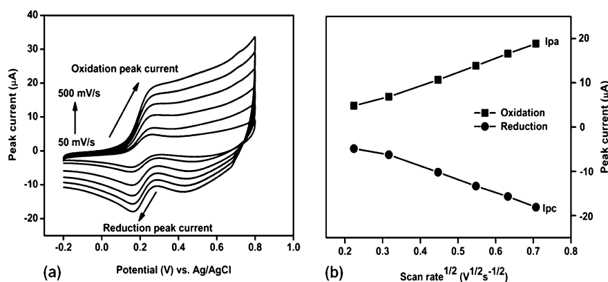
Figure 3. (a) Cyclic voltammograms of \text{Cu}_2\text{O}/\text{Nafion}/\text{GC} electrode in 2 mM \text{K}_3[\text{Fe}(\text{CN})_6] and 0.1 M KCl solution at various scan rates. (b) Plots of anodic and cathodic peak currents vs. scan rate ( I_p vs. \nu^{1/2} ).
