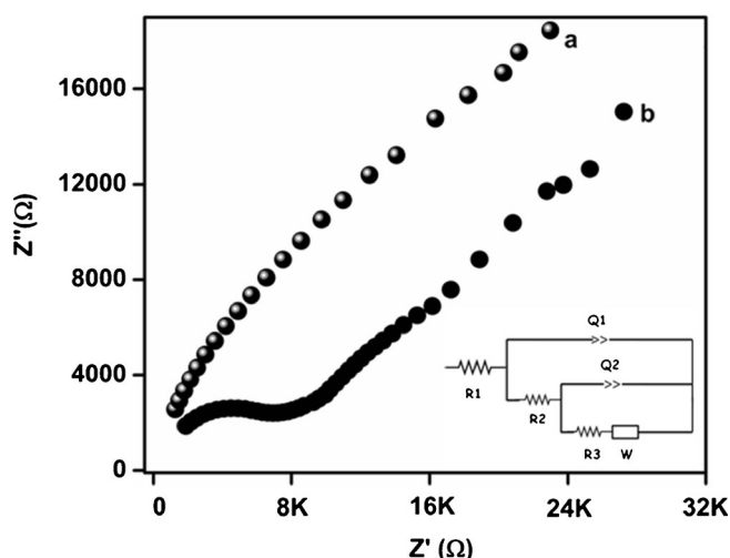
Figure 4. EIS spectrum of the (a) bare GCE and (b) \text{Cu}_2\text{O}/\text{Nafion}/\text{GC} based electrode and its equivalent circuit (inset).
