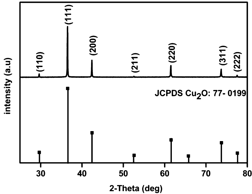
Figure 1. X-ray diffraction pattern of cuprous oxide.
