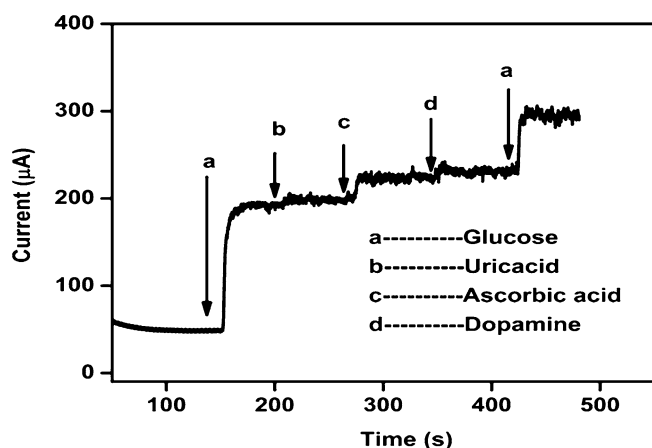
Figure 7. Interference test of \text{Cu}_2\text{O}/\text{Nafion}/\text{GC} electrode modified electrode in 0.1 M NaOH at 0.6 V with 300\mu\text{M} glucose in the presence of 300\mu\text{M} UA, 300\mu\text{M} AA and 300\mu\text{M} DA.
