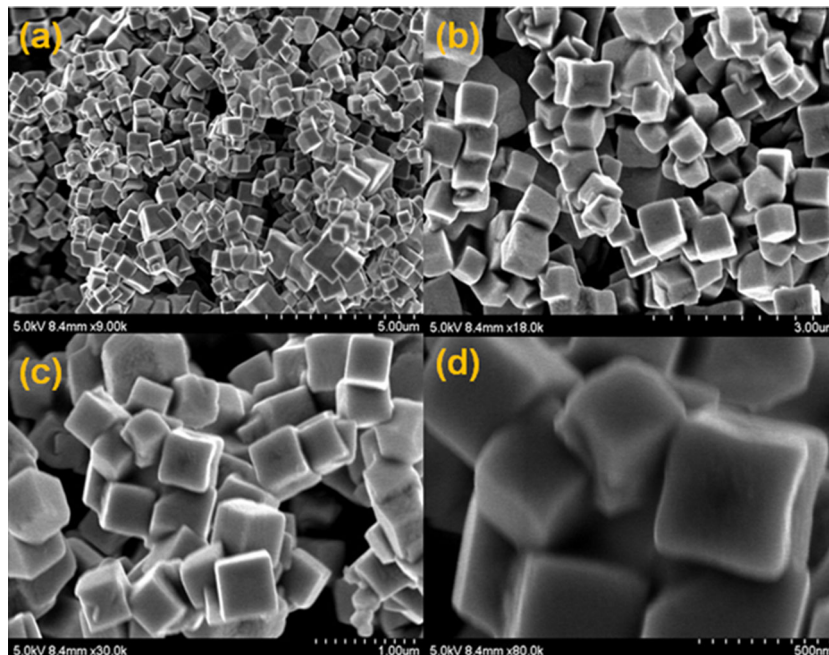
Figure 2. FE-SEM images of cuprous oxide nanostructures at different magnifications.
