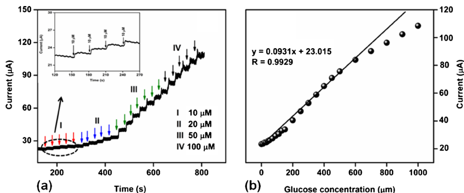
Figure 6. (a) Amperometric steady state current time response obtained at \text{Cu}_2\text{O}/\text{Nafion}/\text{GC} electrode upon successive additions of glucose into 0.1 M NaOH solution. The upper left inset shows the enlarged view at low concentrations of glucose. (b) The linear plot of amperometric current vs. glucose concentrations.
