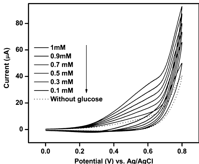
Figure 5. (a) Cyclic voltammetry of \text{Cu}_2\text{O}/\text{Nafion}/\text{GC} electrode in the absence and presence of different concentration of glucose (0.1 mM to 1 mM).
