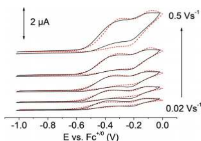
Figure 7. Simulated (black lines) and measured (red dashed lines) CVs of 5 in THF, [n\text{Bu}_4\text{PF}_6] = 0.1 \text{ M} , [\text{N}_2] = 6.4 \text{ mM} , [12] [\text{5}] = 4.0 \text{ mM} .
