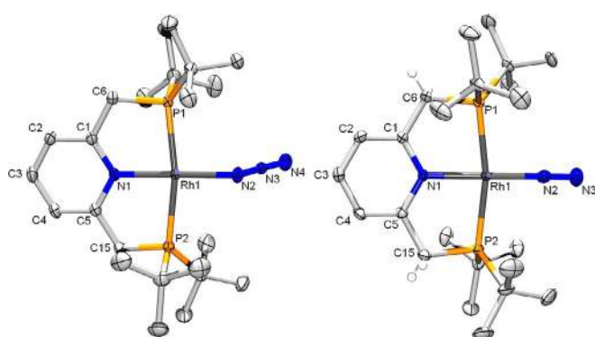
Figure 1. ORTEP plots of the molecular structures of 5 (left) and 9 + (right) (ellipsoids set at 50% probability, hydrogen atoms and PF 6 − anion in 9 + are omitted for clarity). Selected bond lengths [Å] and angles [°]: 5 : Rh1–N1 2.0352(14), Rh1–N2 2.0752(15), Rh1–P1 2.2668(4), Rh1–P2 2.2712(4), P1–C6 1.8449(19), C1–C6 1.505(3), N1–C1 1.364(2), N1–C5 1.368(2), C1–C2 1.387(3), C2–C3 1.379(3); C3–C4 1.380(3), C4–C5 1.384(3), N2–N3 1.195(2), N3–N4 1.166(2), N1–Rh1–N2 178.06(6), P1–Rh1–P2 168.036(18). 9 + : Rh1–N2 1.916(2), Rh1–N1 2.059(2), Rh1–P1 2.3018(7), Rh1–P2 2.3010(7), N2–N3 1.089(3), N1–C1 1.367(3), N1–C5 1.365(3), C1–C2 1.375(4), C2–C3 1.382(4), C3–C4 1.383(4), C4–C5 1.375(4), N1–Rh1–N2 176.15(10), P1–Rh1–P2 167.27(2), Rh1–N2–N3 176.3(3).
