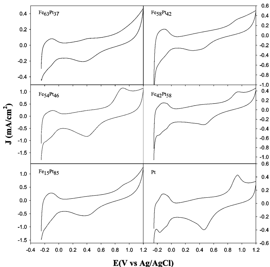
Figure 1. Cyclic voltammograms of the \text{Fe}_x\text{Pt}_{100-x}/\text{GC} electrodes ( x = 63, 58, 54, 42, 15, and 0 ) after UVO treatment in 0.1 \text{ M HClO}_4 . The electrolyte solution was deaerated by ultrahigh-purity nitrogen for 15 min and protected by a nitrogen atmosphere during the entire experimental procedure. Current density was calculated by normalizing the voltammetric currents to the surface area of the glassy carbon electrode. Potential scan rate was 0.1 \text{ V/s} .
