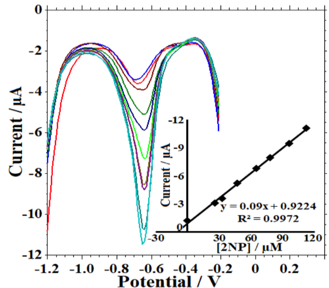
Figure 5. DPVs obtained with 2NP additions in lake water sample and calibration graph (1) pH 2.0 BR buffer (2) Lake water sample, (3) 2NP addition (determined 10 \mu\text{M} 2NP), (4) 26 \mu\text{M} , (5) 33 \mu\text{M} , (6) 47 \mu\text{M} , (7) 65 \mu\text{M} , (8) 78 \mu\text{M} , (9) 96 \mu\text{M} , and (10) 112 \mu\text{M} 2NP.
