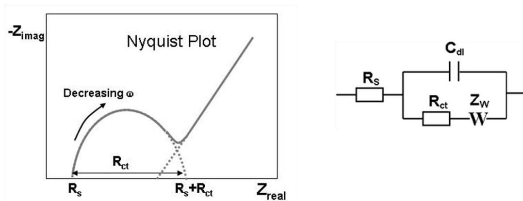
Figure 4. EIS Nyquist plot ( Z_{imag} vs Z_{real} ) and Randles circuit ( W is a so-called Warburg element, which accounts for diffusion processes).
