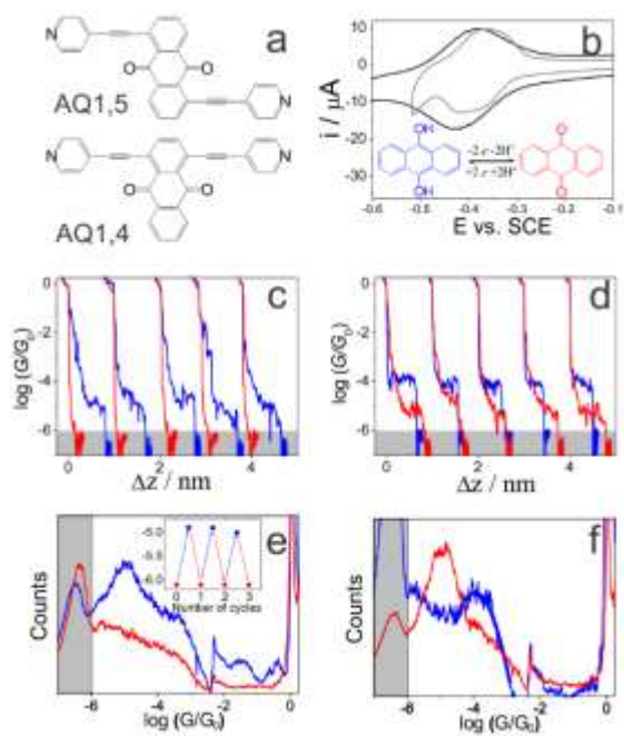
Figure 1. (a) The molecules studied in this work (b) CV of AQ-1,5 (black) and AQ-1,4 (gray) assembly measured in the STM cell with sweep rate of 100 \text{ mV s}^{-1} in 0.1 \text{ M KClO}_4 aqueous electrolyte. (c-d) Typical conductance vs. distance traces of rAQ-1,5 (c, blue), AQ-1,5 (c, red), rAQ-1,4 (d, blue), AQ-1,4 (d, red). The traces for the reduced and oxidized states have been recorded at -530 \text{ mV} and -280 \text{ mV} vs SCE for AQ-1,5 and at -520 \text{ mV} and 280 \text{ mV} for AQ-1,4, respectively. (e-f) 1D conductance histograms generated from 1100 individual curves without any data selection for rAQ-1,5 (e, blue), AQ-1,5 (e, red), rAQ-1,4 (f, blue), AQ-1,4 (f, red). (e, inset) Three sequential in-situ highly reversible switching cycles between rAQ-1,5 and AQ-1,5 triggered by the electrode potential. The data points are the most probable conductances of rAQ-1,5 (blue) and AQ-1,5 (red). The noise level is indicated by the gray area in c-f. The small spike at \log(G/G_0) \approx -2.2 in panels e and f represents an artefact related to the switching of the amplifier. 37
