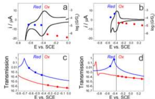
Figure 4. The experimental (a,b) and calculated (c,d) molecular conductance as a function of the applied gating potential vs. SCE for AQ-1,5 (a,c) and AQ-1,4 (b,d). The vertical gray line indicates the measured redox potential for the two molecules. The transmission curves shown in the lower panels are the same as in Figure 2, but are plotted here on the electrochemical energy scale relative to SCE.
