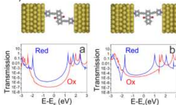
Figure 2. Calculated transmission function for the two charge states of AQ-1,5 (a) and AQ-1,4 (b). The super cells used for the transport calculations are also shown. The energy scale is relative to the Au Fermi level.
