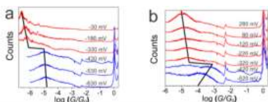
Figure 3. (a-b) Conductance histograms obtained at different potentials vs. SCE for AQ-1,5(a) and AQ-1,4(b). Black lines indicate the conductance changes with electrode potential.
