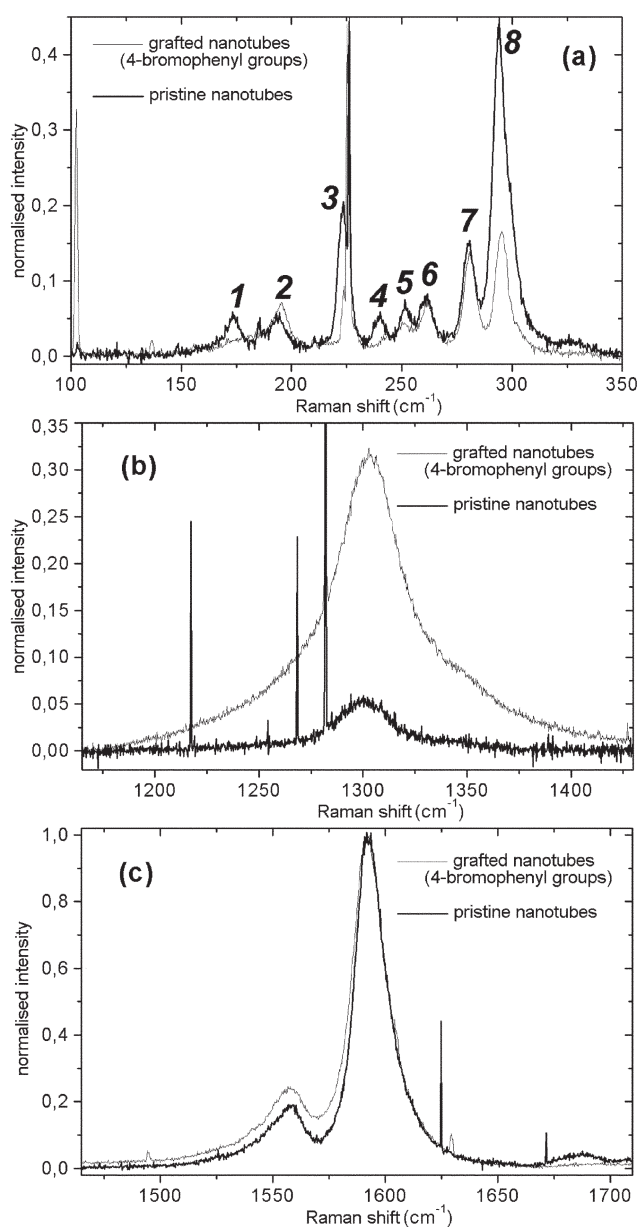
Fig. 3 Micro-Raman diffusion data collected at 676 nm. Intensities are normalized in such a way that the intensity of the strongest tangential mode is 1. Panels a, b and c plot the normalized intensities of, respectively, the radial modes, D-band and tangential modes.
