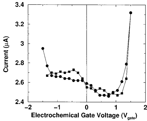
FIG. 2. Current vs electrochemical gate voltage for a nanotube with a fixed 0.5 V bias voltage. The gate voltage is first swept up (circles) from -1.5 to +1.5 V and then down (squares).
