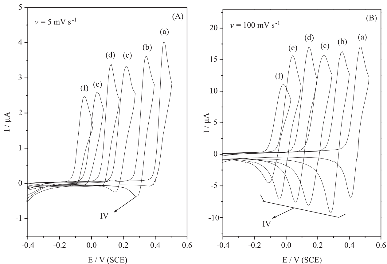
Figure 7. Cyclic voltammograms for 0.8 mmol L -1 quercetin in pH (a) 2.2, (b) 4.4, (c) 6.4, (d) 7.4, (e) 8.4 and (f) 9.2 in hydro-alcoholic solution for (A) 5 and (B) 100 mV s -1 .
