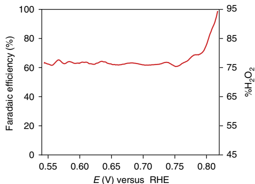
Figure 4 | Faradaic efficiency for H_2O_2 and \%H_2O_2 . Potential-dependent Faradaic efficiency for H_2O_2 production and \%H_2O_2 production during ORR catalysed by \text{Ni}_3(\text{HITP})_2 at pH 13.
