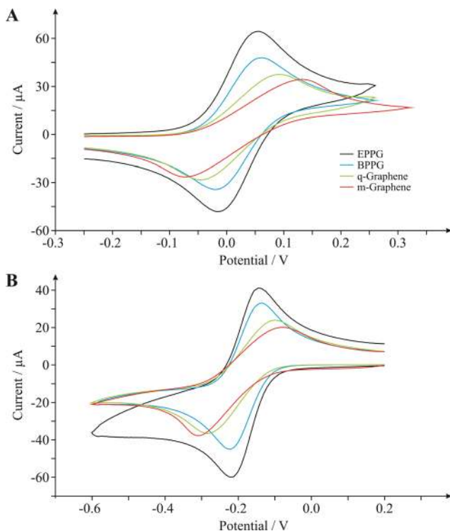
Fig. 8 Cyclic voltammograms obtained using (A) N,N,N',N' -tetramethyl- para -phenylenediamine (TMPD) and (B) hexamine-ruthenium(III) chloride at EPPG (black), BPPG (blue), quasi -graphene ( q -graphene, green) and monolayer graphene ( m -graphene, red) electrodes. Scan rate shown for each electrode: 100 mV s -1 (vs. SCE).
