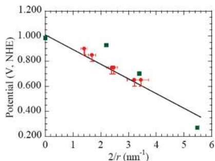
Figure 4. Influence of Pt particle size ( 2/r ) on the dissolution potential ( V_{\text{diss}} ). Red points are experiment. Vertical error bars correspond to \sim 50 mV, and horizontal error bars indicate measurement errors of \sim 8\% . A linear fit to these data yields V_{\text{diss}} = 1.067 - 0.127(2/r) V. The black line is the thermodynamic prediction of the Gibbs–Thomson equation, V_{\text{diss}} = 1.011 - 0.111(2/r) V. The green squares are the ab initio results.
