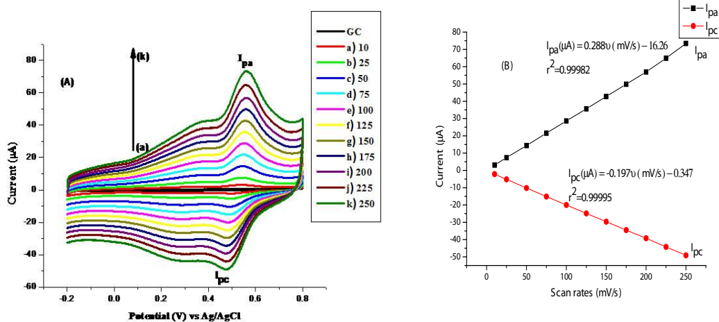
Fig. 2: Cyclic voltammograms of LG/GC electrode recorded at scan rates of 10 – 250 mV/s (inner to outer) in 0.1 M \text{HNO}_3 (A), plot of peak currents vs. scan rates (B)
