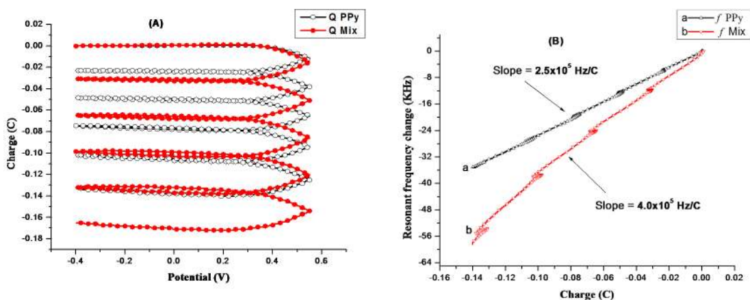
Fig. 12: Plots of charge response vs. potential (A) and resonant frequency change responses as function of charge passed for the deposition of the PPy (a) and composite (b) films (B) at a gold-coated quartz crystal electrode for 5 consecutive potential cycles in 1.0 M sulfuric acid
