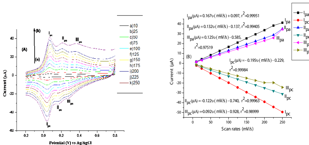
Fig. 2: Cyclic voltammograms of LG/GC electrode recorded at scan rates of 10 – 250 mV/s (inner to outer) in 0.1 M \text{HNO}_3 (A), plot of peak currents vs. scan rates (B)
