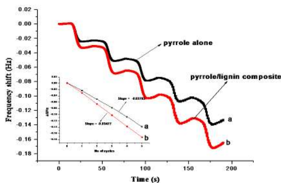
Fig. 13: Plots of frequency shift as a function of time and frequency shift as a function of number of cycles (inset plot) for pyrrole (a) and pyrrole/lignin composite (b) in 1.0 M sulfuric acid
