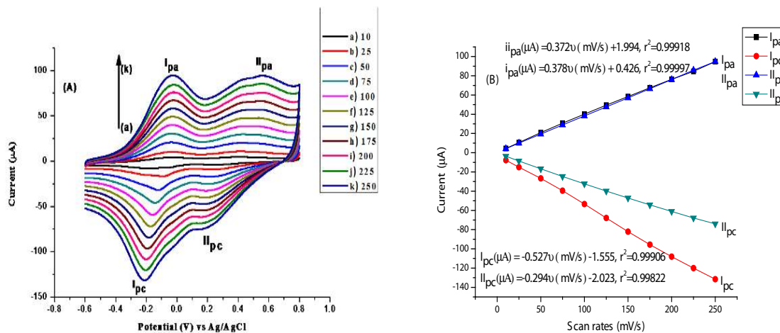
Fig. 7: Cyclic voltammograms of LG-co-OPDA/GC composite film modified electrode recorded at scan rates of 10 – 250 mV/s (inner to outer) in 0.1 M HNO_3 (A), graphs of peak currents on its scan rates
