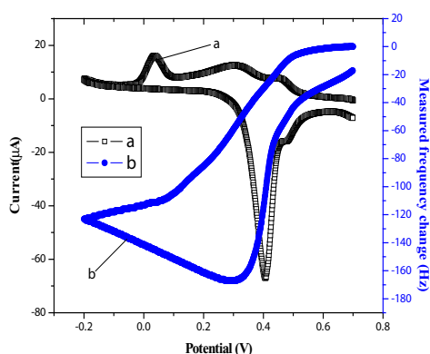
Fig. 10: Potentiodynamic deposition and dissolution of 1.0 mM silver nitrate in 1.0 M sulfuric acid, (a) current vs. potential curve and (b) measured frequency change vs. potential curve
