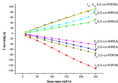
Fig. 8: Peak current comparison between LG-co-AHNSA/GCE and LG-co-POPDA/GCE composite films modified electrodes at a scan rate of 10 – 250 mV/s in 0.1M HNO_3 supporting electrolyte solution
