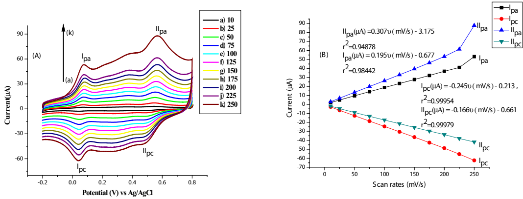
Fig. 4: Cyclic voltammograms of LG-co-AHNSA/GCE composite film modified electrode recorded at scan rates of 10 – 250 mV/s (inner to outer) in 0.1 M HNO 3 (A), plots of peak current vs. scan rate and their square roots for (B) and (C), respectively
