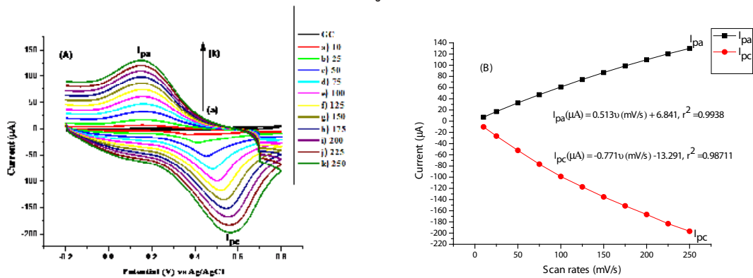
Fig. 6: Cyclic voltammograms of POPDAIGC modified electrode recorded at scan rates of 10 – 250 mV/s (inner to outer) in 0.1 M HNO 3 (A), plot of peak currents on scan rates (B)
