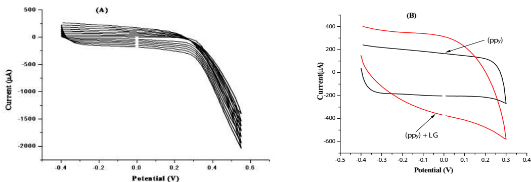
Fig. 9: Cyclic voltammograms of electropolymerization of pyrrole (A) peak comparison of CVs poly pyrrole with lignin composites (LG + PPy) and pure polypyrrole modified electrode (B) in the potential range from -0.4 to +0.3 V: 1.0 M H_2SO_4 as supporting electrolyte
