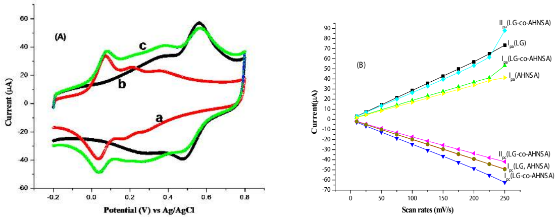
Fig. 5: Cyclic voltammograms of a) 2 mM AHNSA, b) 10 mg/ml of LG, and c) composite films, scan rate 200 mV/s (A) their peak current dependence at a scan rates of 10 – 250 mV/s in 0.1 M HNO 3 supporting electrolyte solution (B)
