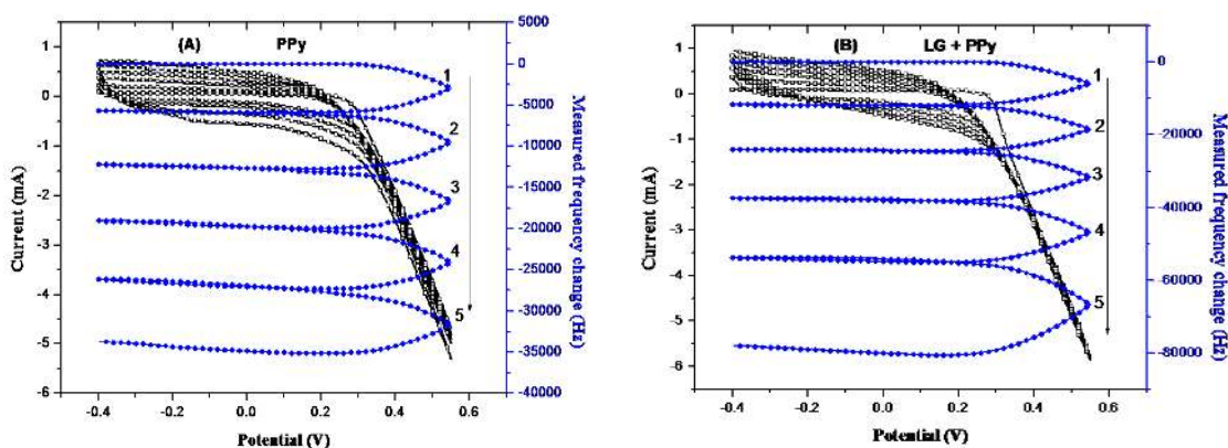
Fig. 11: Potentiodynamic polymerization of pyrrole (A) and pyrrole/lignin composite (B) (current vs. potential) at a gold-coated quartz crystal electrode for 5 consecutive potential cycles and the Frequency shifts recorded in 1.0 M sulfuric acid
