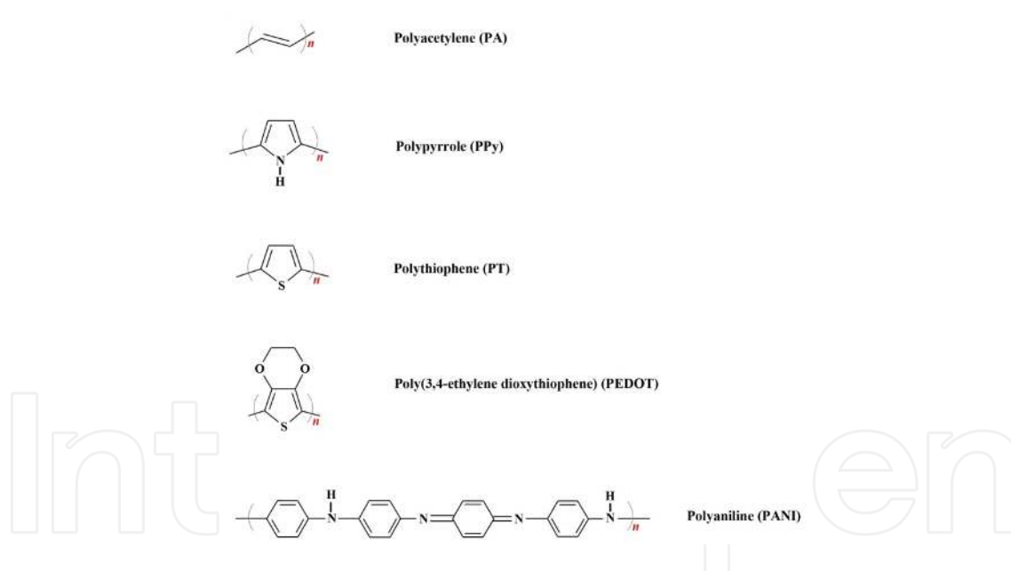
Figure 1. Chemical structures of various conducting polymers
