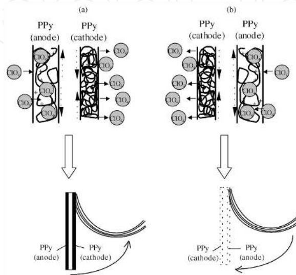
Figure 6. The triple layer device (polypyrrole( \text{ClO}_4^- )/non-conducting and adherent polymer/polypyrrole( \text{ClO}_4^- )) and its macroscopic movement produced as a consequence of volume change in the polypyrrole films. (a) A current flows and the left polypyrrole film acting as the anode is swelled by the entry of the hydrated counter ions ( \text{ClO}_4^- ). Simultaneously, the right film acting as the cathode contracts and shrinks because of the expulsion of the counter ions. These volume changes and the constant length of the non-conducting film promote the movement of the triple layer towards the polypyrrole film that is being contracted. (b) By changing the direction of the current, the movement takes place in the opposite direction. The muscle works in \text{LiClO}_4 aqueous solution [83]
