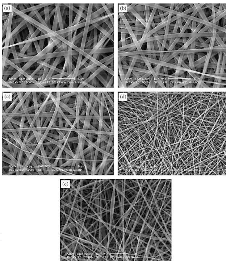
Figure 8. SEM micrographs of gelatin fibers (a) and PANI-gelatin blend fibers with ratios of (b) 15:85; (c) 30:70; (d) 45:55; and (e) 60:40. Original magnifications are 5000× for (a–d) and 20000× for (e). Figure shows the electrospun fibers were homogeneous while 60:40 fibers were electrospun with beads [90]
