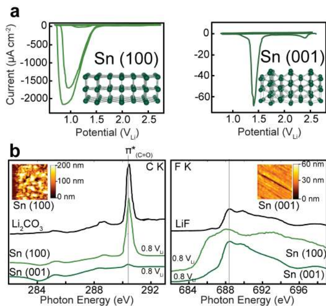
Figure 5. a) CV measurements on tetragonal \beta -Sn (100) and \beta -Sn (001) from 2.8 to 0.8 V_{\text{Li}} at 1\text{mV s}^{-1} in 1\text{M LiPF}_6 , EC:DEC 1:2 electrolyte, showing higher cathodic current for \beta -Sn (100). 132 The inserts show atomic arrangement of the tetragonal \beta -Sn (100) and (001) surfaces, respectively. b) C-K (left) and F-K (right) edge Soft X-ray Absorption Spectroscopy (XAS) of the SEI on the \beta -Sn(100) and (001) surfaces after few CV between 0.8-2.5 V_{\text{Li}} (note that 0.8 V_{\text{Li}} is above the lithiation potential of Sn). 132 The \beta -Sn(100) consists mostly of porous carbonate while the \beta -Sn(001) consists mostly of LiF. The inserts are in situ AFM images of the \beta -Sn(100) and (001) surfaces at 2.5 V_{\text{Li}} after cycling twice from 2.5 V_{\text{Li}} to 0.8 V_{\text{Li}} , 185 showing that the SEI on the (100) surface is rougher and thicker than the (001). 185
