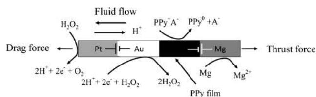
Fig. 7 Catalytic nanomotors for a self-powered drug delivery system. After Pumera [71] and Sundararajan et al. [89]
