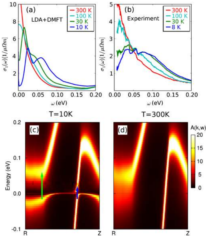
FIG. 43 (color online). The development of the hybridization gap in the heavy-fermion compound \text{CeIrIn}_5 . (a) The optical conductivity calculated by LDA+DMFT method. From Shim et al. , 2007. (b) Experimental optical conductivity for the same compound measured by Mena et al. (2005). (c) Theoretical momentum-resolved non- f spectral function at low temperature. The two types of hybridization gaps are marked by arrows in (c). (d) Same as (c) but for higher temperature.
