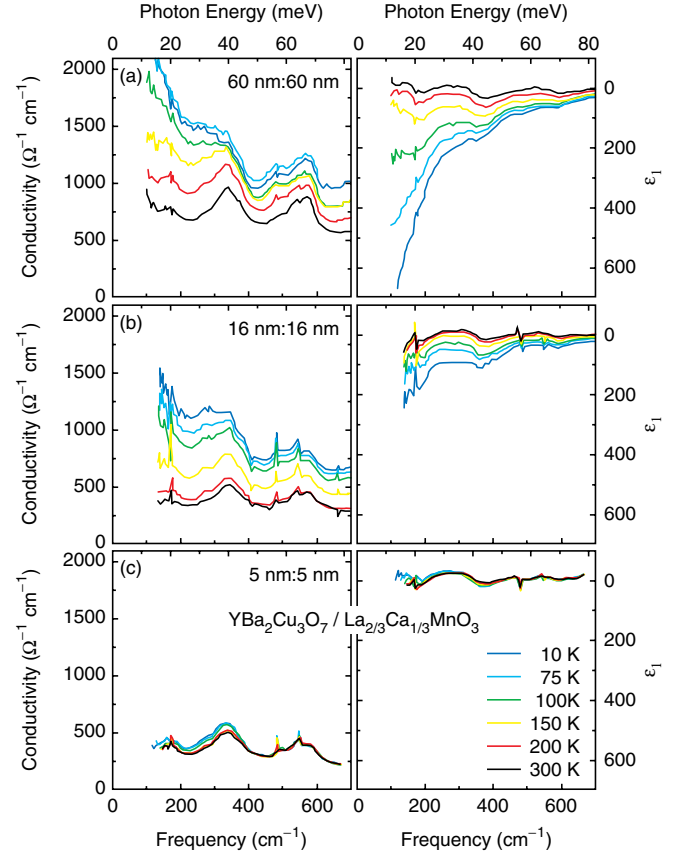
FIG. 39 (color online). Optical conductivity and dielectric constant of superlattices consisting of equal thickness of YBCO and LCMO layer. The thickness of each layer in (a), (b), and (c) is 60, 16, and 5 nm, respectively. From Holden et al. , 2004.
