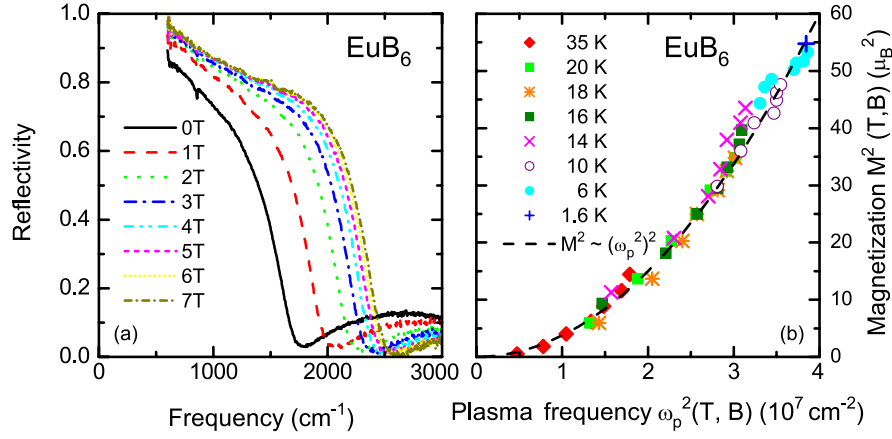
FIG. 45 (color online). (a) Magneto-optical reflectivity of EuB 6 at 16 K; (b) scaling of magnetization and plasma frequency. From Broderick et al. , 2002.
