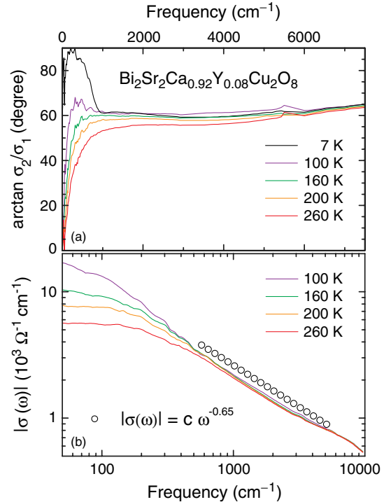
FIG. 12 (color online). Universal power law of the optical conductivity and the phase angle spectra of optimally doped \text{Bi}_2\text{Sr}_2\text{Ca}_{0.92}\text{Y}_{0.08}\text{Cu}_2\text{O}_8 . (a) The phase function of the optical conductivity \arg\{\sigma(\omega)\} . The error margins of \epsilon_\infty = 4.5 \pm 0.5 propagate to an uncertainty of \pm 2^\circ of the phase of \sigma(\omega) for \omega = 5000\text{ cm}^{-1} . (b) The absolute value of the optical conductivity is plotted on a double logarithmic scale. The open symbols correspond to the power law |\sigma(\omega)| = C\omega^{-0.65} . From van der Marel et al. , 2003.
