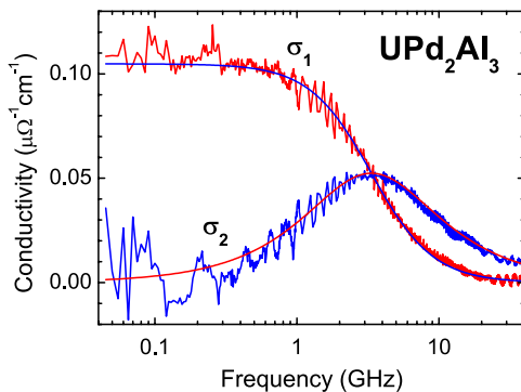
FIG. 7 (color online). Optical conductivity spectrum (real and imaginary parts) of UPd 2 Al 3 at temperature T = 2.75 K. The fit by Eq. (1), with \sigma_{dc} = 1.05 \times 10^5 (\Omega \text{ cm})^{-1} and \tau = 4.8 \times 10^{-11} s, documents the excellent agreement of experimental data and the Drude prediction. The characteristic relaxation rate 1/(2\pi\tau) is marked by the decrease in \sigma_1 and the maximum in \sigma_2 around 3 GHz. From Scheffler et al. , 2005.
