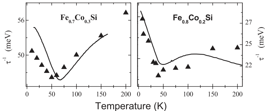
FIG. 46. Temperature dependence of the optical scattering rates \hbar/\tau (triangles) of Fe 1-x Co x Si for two different doping concentrations, and dc resistivities scaled as to overlay the scattering rates (solid curves). From Mena et al. , 2006.
