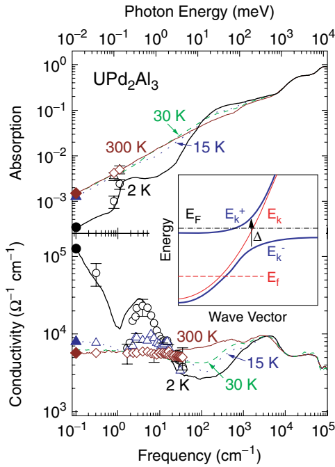
FIG. 40 (color online). Frequency-dependent absorptivity A(\omega) = 1 - R(\omega) and optical conductivity of UPd 2 Al 3 at different temperatures shown over a wide frequency range. The solid symbols on the left axis are from dc measurements; the open symbols in the microwave range are obtained by cavity perturbation technique. In the terahertz range the optical conductivity is determined directly using the transmission and the phase shift measured by the Mach-Zehnder interferometer. The lines are from various optical investigations [transmission through films and reflection of bulk samples (Degiorgi, Dressel et al. , 1994)] and simultaneously match the directly measured conductivity and dielectric constant (Dressel, Kasper, Petukhov, Gorshunov et al. , 2002, Dressel, Kasper, Petukhov, Peligrad et al. , 2002). Inset: Renormalized band structure calculated from the Anderson lattice Hamiltonian. E_k and E_f denote bands of free carriers and localized f electrons. At low temperatures, a direct gap \Delta opens. The Fermi level E_F is near the bottom of the upper band E_k^+ , resulting in enhanced effective mass of the quasiparticles.
