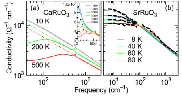
FIG. 11 (color online). (a) Temperature-dependent \sigma_1(\omega) of \text{CaRuO}_3 shows the power-law scaling at three representative temperatures. The symbols in the inset mark the energy scale where power law \omega^{-1/2} ceases to hold. From Y.S. Lee et al. , 2002. (b) Logarithmic plot of \sigma_1(\omega) for \text{SrRuO}_3 . The curves from the top correspond to temperatures T = 8\text{ K} , 40\text{ K} , 60\text{ K} , and 80\text{ K} , respectively. Dotted lines are fits to Eq. (27). From Dodge et al. , 2000b.
