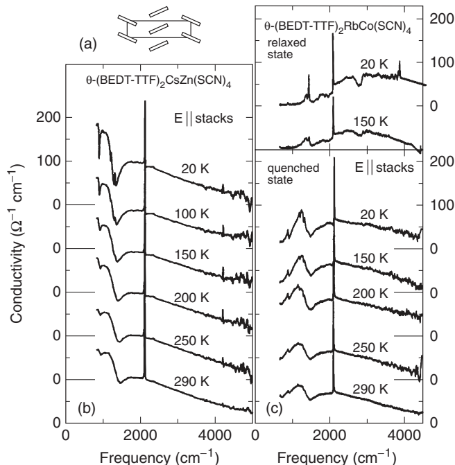
FIG. 54. (a) The structural arrangement of the \theta phase reveals two stacks of BEDT-TTF molecules in a herringbone fashion. Optical conductivity of (b) \theta -(BEDT-TTF) _2 CsZn(SCN) _4 and (c) \theta -(BEDT-TTF) _2 RbCo(SCN) _4 measured along the stacks ( c axis) for different temperatures. The charge-ordered state in the latter is only reached when slowly cooled (0.1 K/min), for rapid cooling (1 K/min) the crystal remains metallic (Tajima et al. , 2000). The curves for different temperatures are displaced.
