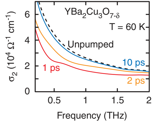
FIG. 27 (color online). Imaginary part of the far-infrared conductivity in a \text{YBa}_2\text{Cu}_3\text{O}_{7-\delta} film as a function of frequency for various times following photoexcitation. An initial reduction in the condensate density yields a reduction in the 1/\omega response which recovers in \sim 2 ps. From Averitt, Rodriguez et al. , 2001.
