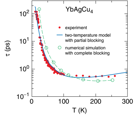
FIG. 41 (color online). Temperature dependence of the relaxation time on YbAgCu 4 . Numerical simulations have been performed assuming suppressed scattering of heavy electrons by phonons; the solid line corresponds to simulations by a two-temperature model with a partial reduction of the scattering. An equally good description is obtained by coupled Boltzmann equations when the electron-phonon coupling is suppressed for electronic states within the Abrikosov-Suhl peak in the density of states (Demsar, Averitt et al. , 2003; Ahn et al. , 2004).
