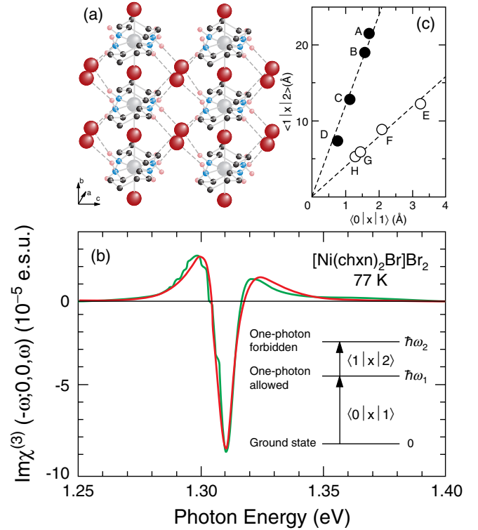
FIG. 49 (color online). (a) Arrangement of the Ni and Br ions along chains in [Ni(chxn) 2 Br]Br 2 leads to an overlap of the Ni 3d z 2 and Br 4p z orbitals. From Takaishi and Yamashita, 2008. (b) \text{Im}\chi^{(3)}(-\omega; 0, 0, \omega) spectra of [Ni(chxn) 2 Br]Br 2 at T = 77 K. The lines are the experimental and calculated results. The energy levels are sketched in the lower panel. (c) Relation between the transition dipole moments of \langle 0|x|1 \rangle and \langle 1|x|2 \rangle for one-dimensional Mott insulators [solid circles: A, [Ni(chxn) 2 Br]Br 2 ; B, [Ni(chxn) 2 Cl]Cl 2 ; C, [Ni(chxn) 2 Cl](NO 3 ) 2 ; D, Sr 2 CuO 3 ] compared to other one-dimensional materials; [empty circles: E, [Pt(en) 2 ][Pt(en) 2 I 2 ](ClO 4 ) 4 ; F, [Pt(en) 2 ][Pt(en) 2 Br 2 ](ClO 4 ) 4 ; G, [Pt(en) 2 ][Pt(en) 2 Cl 2 ](ClO 4 ) 4 ; H, polydiethylsilane (PDHS)]. From Kishida et al. , 2000.
