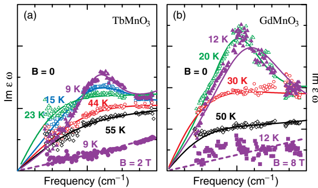
FIG. 37 (color online). Frequency dependence of the imaginary parts of the terahertz-dielectric function in (a) \text{TbMnO}_3 and (b) \text{GdMnO}_3 with e \parallel a and b \parallel c . Open symbols represent experimental data in zero external magnetic field and in the IC-AFMR phase. Solid lines represent model calculations adding an overdamped Lorentzian (dashed lines) to the residual high-frequency contribution. Filled spheres represent the data in the CA-AFMR state obtained by applying B = 2 \text{ T} ( \text{GdMnO}_3 ) and B = 8 \text{ T} ( \text{TbMnO}_3 ) along the c axis. The corresponding zero-field data are shown by filled triangles. From Pimenov, Mukhin et al. , 2006.
