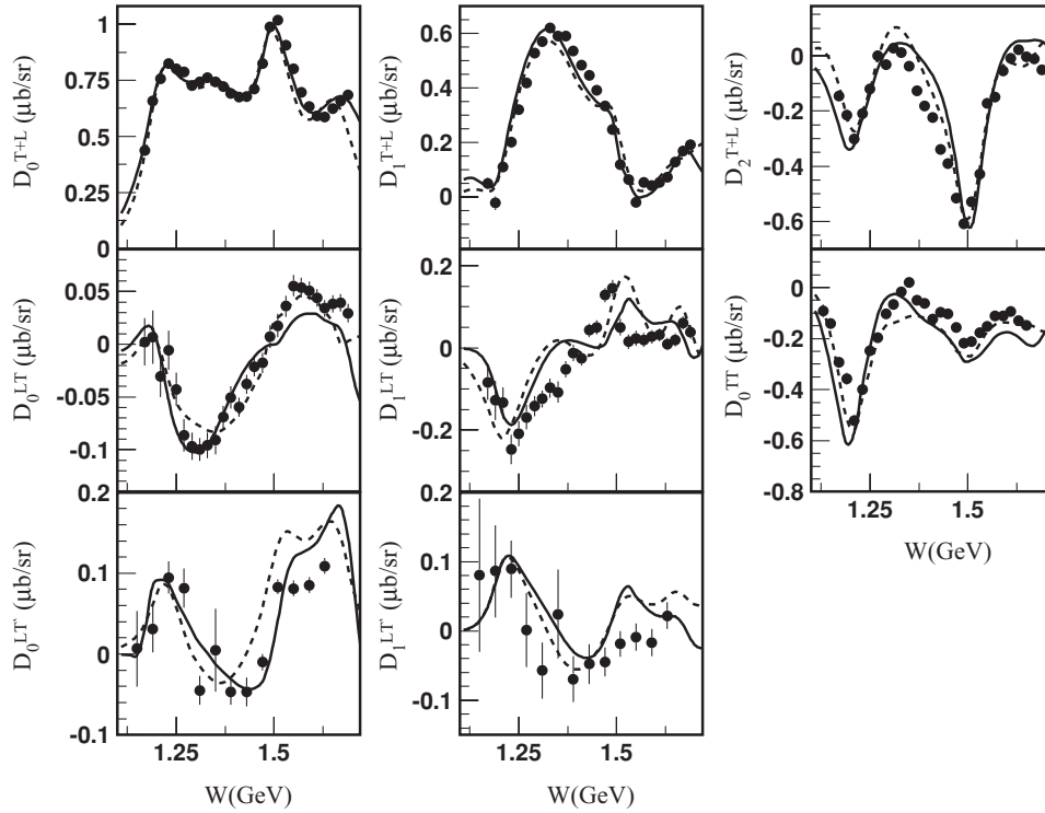
FIG. 5. Our results for the Legendre moments of the \bar{e}p \rightarrow e n \pi^+ structure functions in comparison with experimental data [7] for Q^2 = 2.44 \text{ GeV}^2 . The solid (dashed) curves correspond to the results obtained using the DR (UIM) approach.
