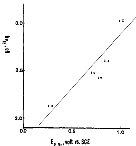
Figure 8. Energy of exciplex emission maximum vs. peak potential for oxidation of donor for ecl of naphthalene with various donors in ACN. See Table III for donor molecules.
