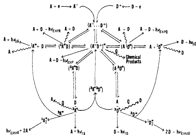
Figure 9. Schematic diagram for reaction paths in ecl. Heavy arrows represent radiative transitions and energy of species decrease (approximately) on proceeding from top to bottom of the figure.
