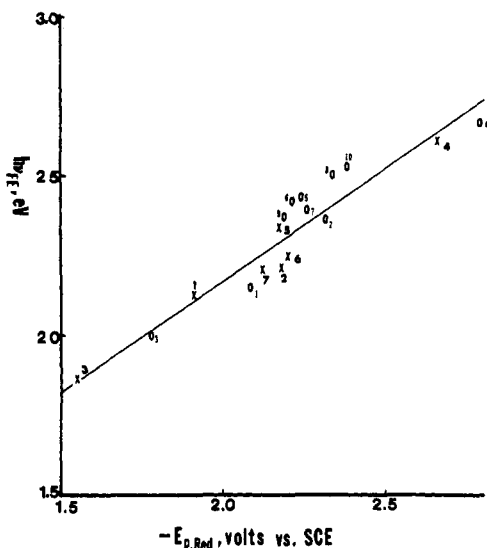
Figure 7. Energy of exciplex emission maximum vs. peak potentials for reduction of acceptor for ecl of TPTA with various acceptors in THF (O) and ACN (X) solutions. The numbers indicate acceptor molecules listed in Table I.
