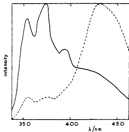
Figure 1. Spectra (uncorrected) of thermoluminescence of 10^{-2} molar zone-refined trans -stilbene in squalane after 2 min of \gamma irradiation: (—) early in glow peak; (- - -) late in glow peak.
