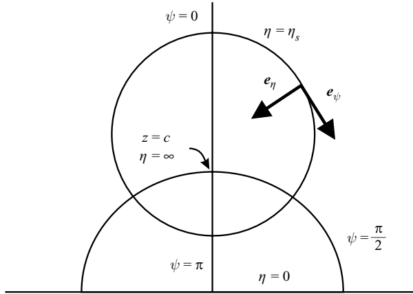
FIGURE 5. Definition sketch for the bispherical coordinate system.
