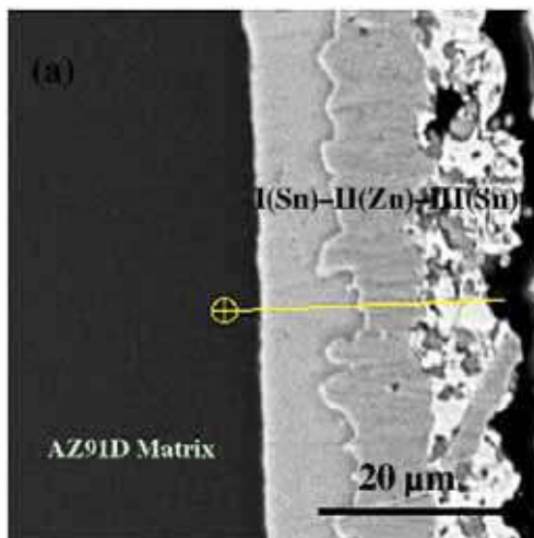
Fig. 27. Cross-section image of the Zn-Sn plated coating on AZ91D alloy after thermal treatment at 190°C for 12 h (Zhu et al., 2006).
