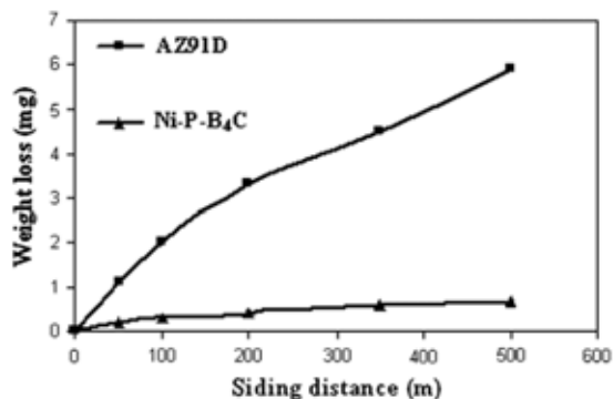
Fig. 16. Weight loss as a function of distance for both substrate and 50 μm thickness Ni-P-B 4 C composite coating obtained from pin-on-disc test (Araghi and Paydar, 2010).
