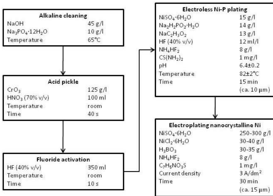
Fig. 23. Flowchart of the electroless Ni and electroplated nanocrystalline Ni on the AZ91D magnesium alloy (Gu et al., 2005 and 2006).
