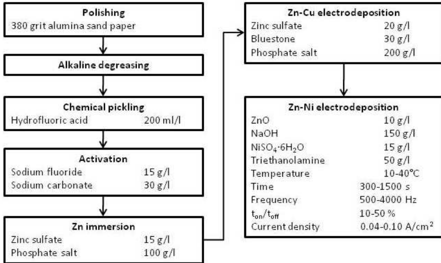
Fig. 28. Flowchart of the Zn-Ni electroplating process on the AZ91D magnesium alloy (Jiang et al., 2005b).
