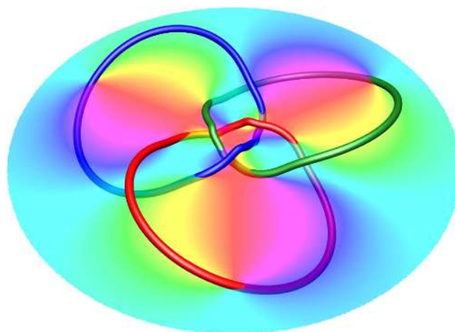
Figure 2. Three optical vortex loops forming Borromean rings, unlinked pairwise but linked triply. (Courtesy of Robert King.)
