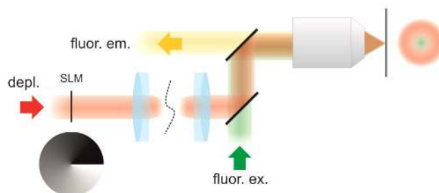
Figure 13. Examples of microscopy methods structuring light on the illumination side: structured illumination microscopy (SIM), STED.
