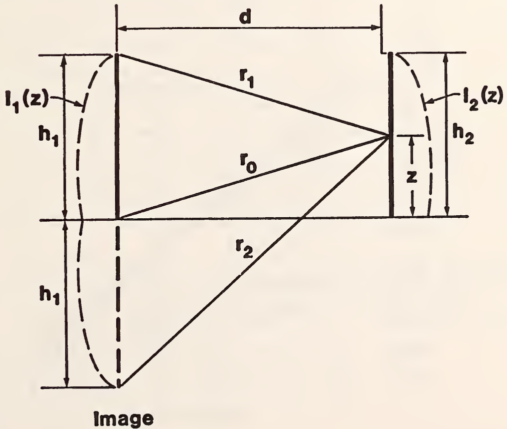
Figure 2.2. Computation of mutual impedance.
