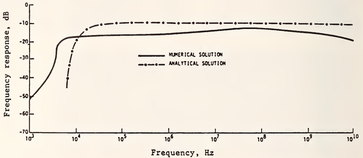
Figure 7.9 Frequency response of a typical probe-diode system with E_{inc} = 1 V/m.
