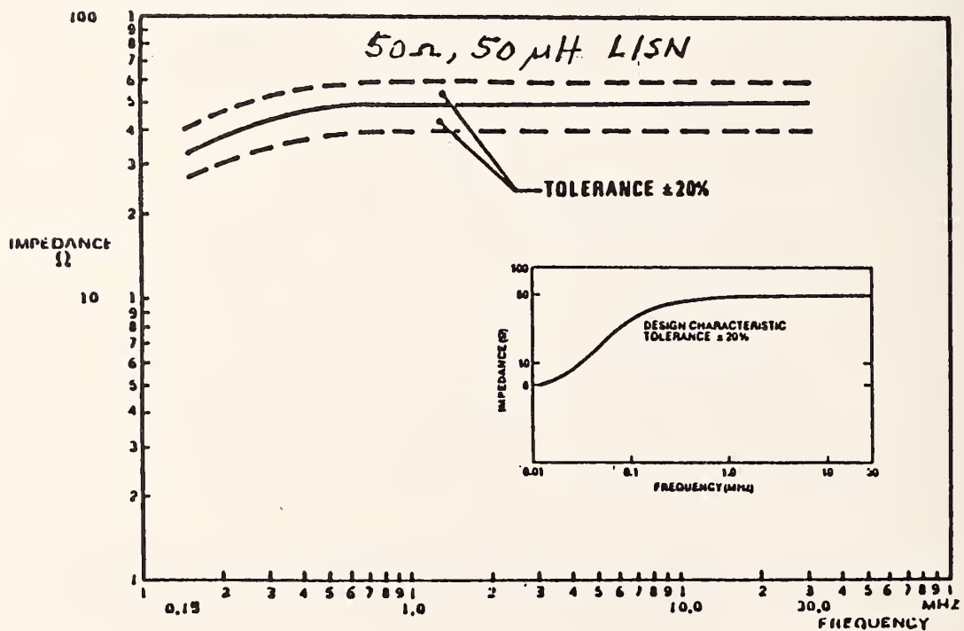
Figure 9.c.13 Line-impedance characteristic (inset) for making conducted emission measurements, as mandated by FCC Docket 20780, (from [1] and [18]).
