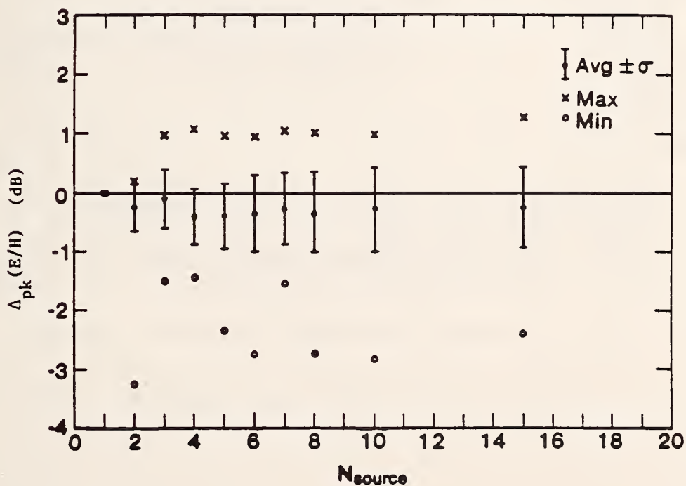
Figure 9.a.6 Mean, standard deviation, and maximum and minimum values of \Delta_{pk}(E/H) , using 100 random configurations for each N_{source} .
