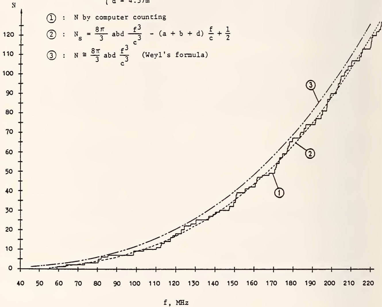
Figure 8.1 Total number of modes as a function of operating frequency for the NBS chamber.
