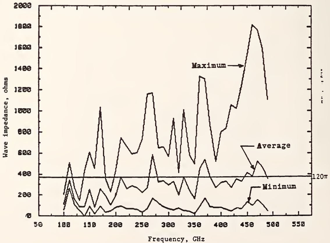
Figure 8.18 Wave impedance of the NBS chamber.
