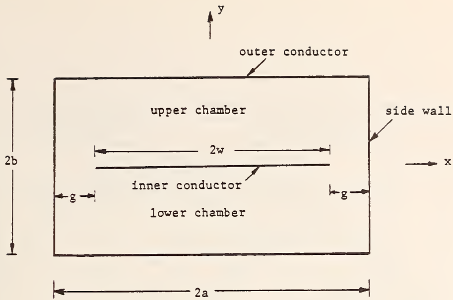
Figure 3.2 Cross section of a TEM cell.
