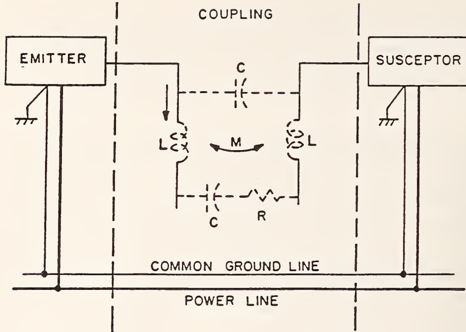
Figure 9.c.2 Ground line and reactance-coupled CEMI.
