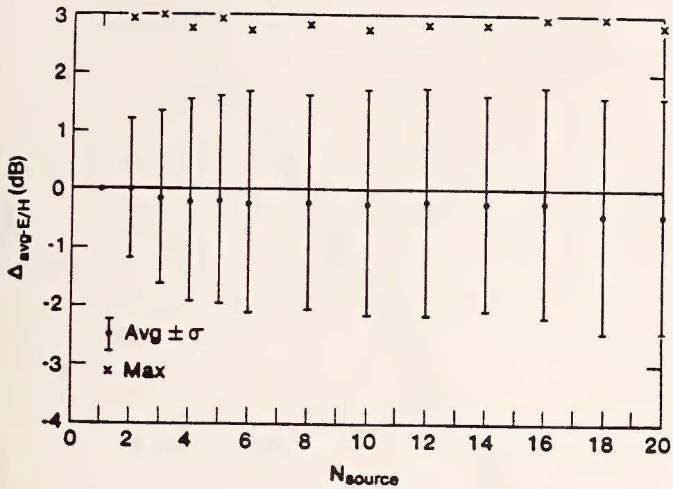
Figure 9.a.5 Mean, standard deviation, and maximum values of the error \Delta_{avg}(E/H) , as functions of the number of sources. For each N_{source} , 1000 random configurations were used.
