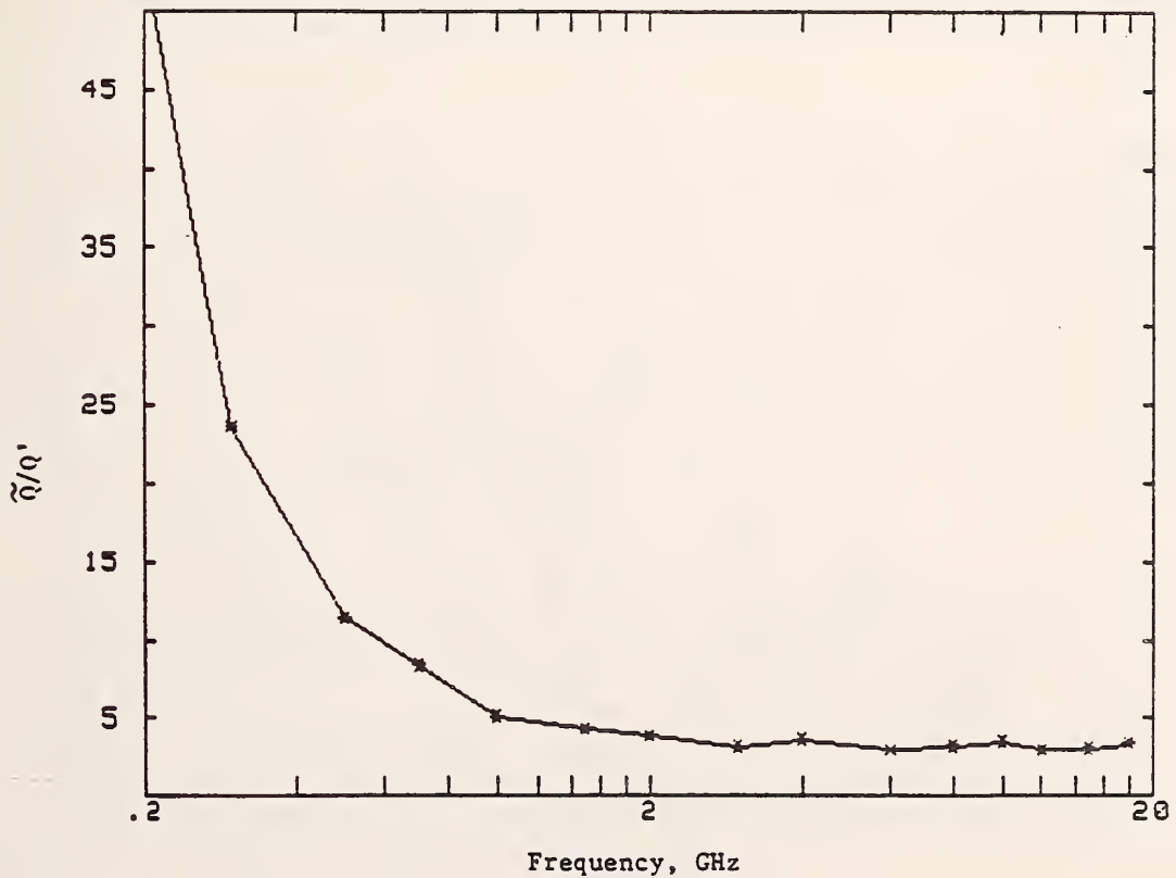
Figure 8.16 Ratio of theoretical composite \tilde{Q} to experimental mean Q' .
