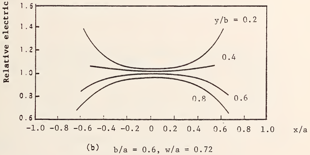
Figure 3.5 Normalized magnitude of the electric field of the TEM mode inside an RCTL.
