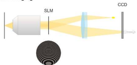
Figure 14. Examples of microscopy methods structuring light on the detection side: Fourier filtering, multiplexing.
