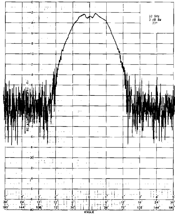
Figure 14. Antenna Patterns for Unhooded ASN 116A Antenna at 7, 8, 9 and 10 GHz.
