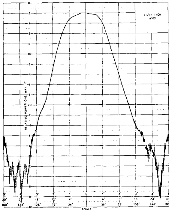
Figure 15. Antenna Patterns for ASN 111A Antenna at 4 GHz.
