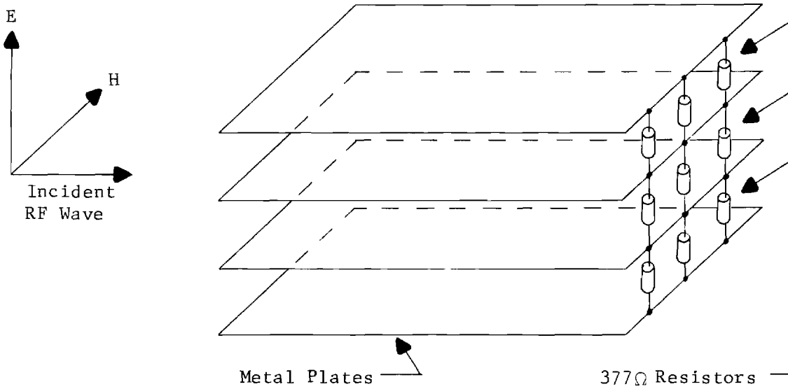
Figure 73. Parallel Plate Absorbing Material
