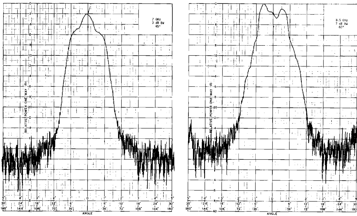
Figure 19. Antenna Patterns for Hooded ASN 111A Antenna at 7 and 8.5 GHz.
