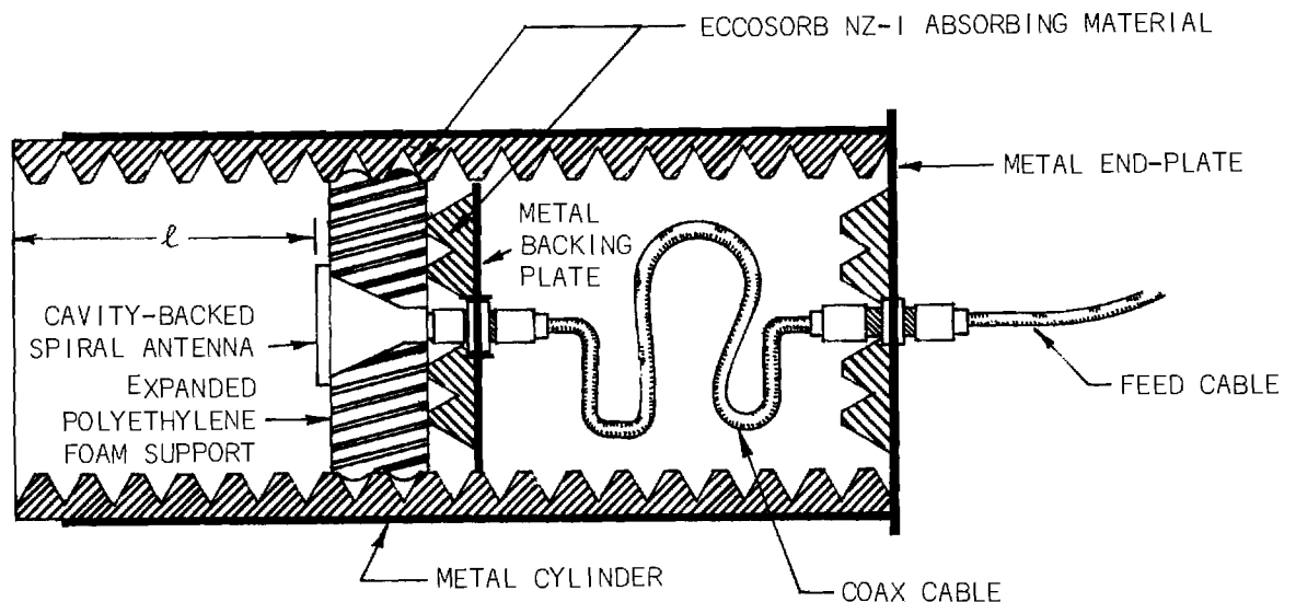
Figure 11. Diagram of Adjustable-Length Hooded Antenna.
