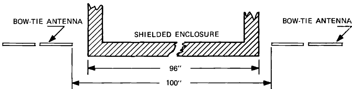
(B) MEASUREMENT SETUP FOR PHASE MEASUREMENTS
