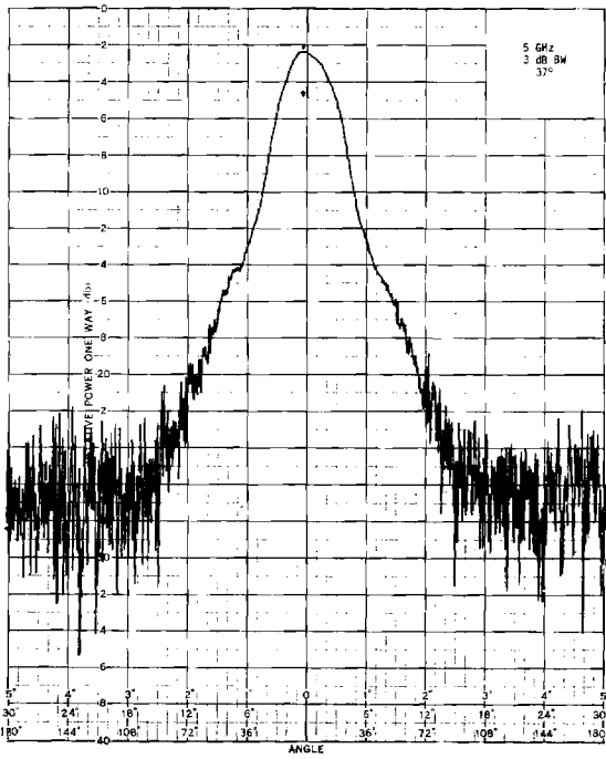
Figure 18. Antenna Patterns for Hooded ASN 111A Antenna at 3, 4, 5 and 6 GHz.
