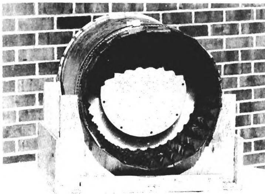
Figure 12. Adjustable-Length Hooded ASN 116A Antenna.
