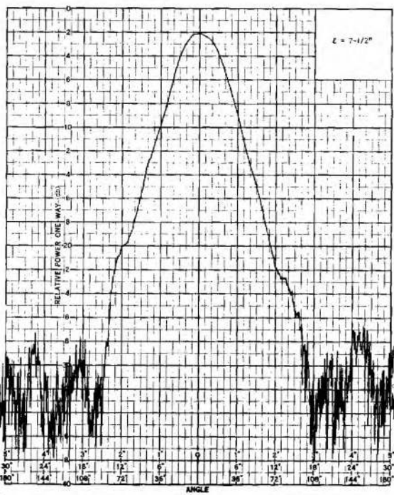
Figure 12. Patterns of Hooded Antenna as a Function of Hood Length at 2 GHz.
