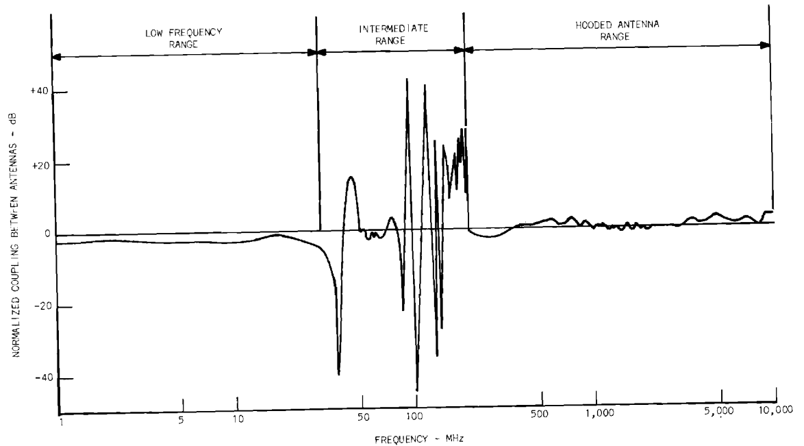
Figure 4. Coupling Between Antennas in a Shielded Enclosure at 1 Meter Separation over the Frequency Range from 1 MHz to 10 GHz.
