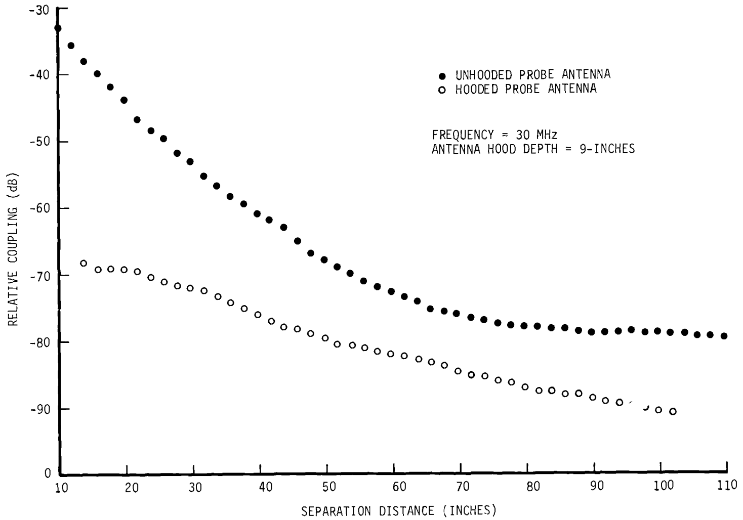
Figure 8. Open-Field Relative Coupling at 30 MHz.
