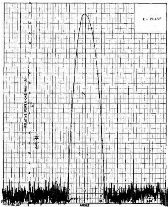
Figure 14. Patterns of Hooded Antenna as a Function of Hood Length at 6 GHz.
