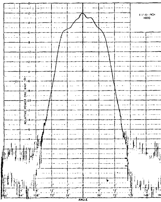
Figure 18. Antenna Patterns for ASN 111A at 10 GHz.
