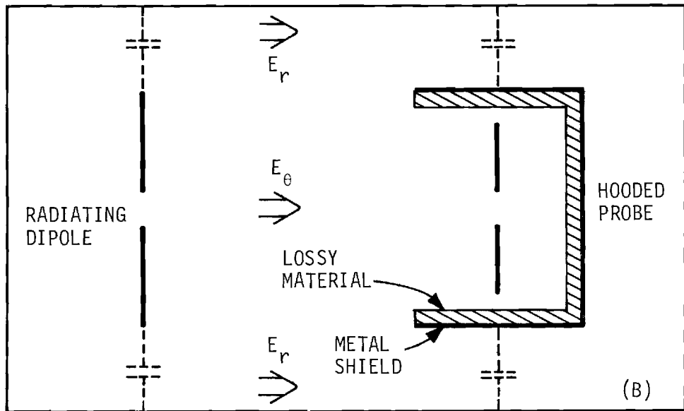
Figure 1. Illustration of the Use of an Antenna Hood to Minimize Probe Response to Radially Polarized Fields.
