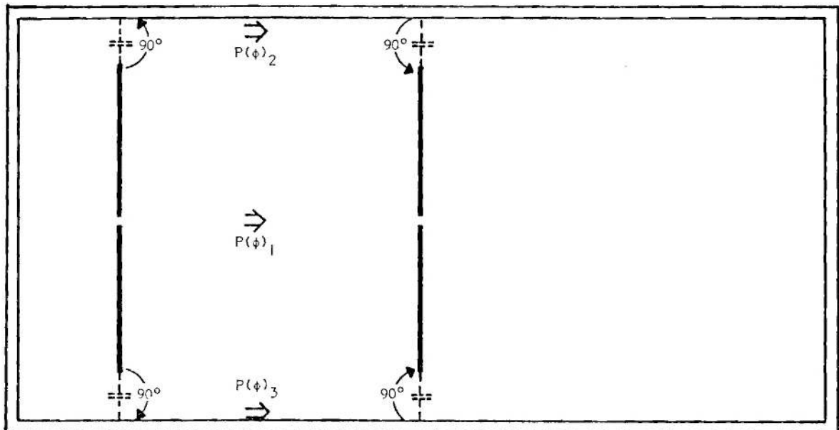
Figure 2. Diagram Showing Primary Paths Between Two Dipole Antennas in a Shielded Enclosure at Low Frequencies.
