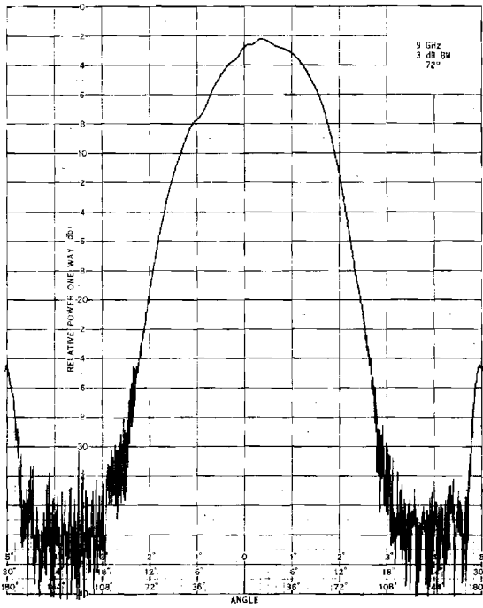
Figure 14. Antenna Patterns for Unhooded ASN 116A Antenna at 7, 8, 9 and 10 GHz.
