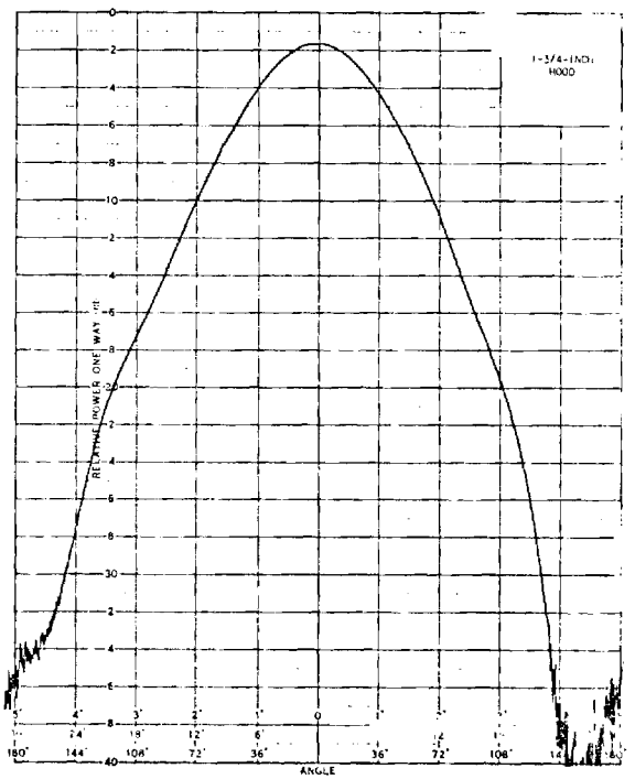
Figure 9. Antenna Patterns for AEL Model ASN 112A Cavity-Backed Spiral Antenna at 1 GHz.
