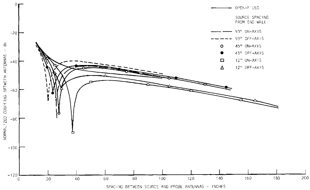
Figure 6. Coupling Between Antennas as a Function of Spacing and Source Location in a Shielded Enclosure at 50 MHz.
