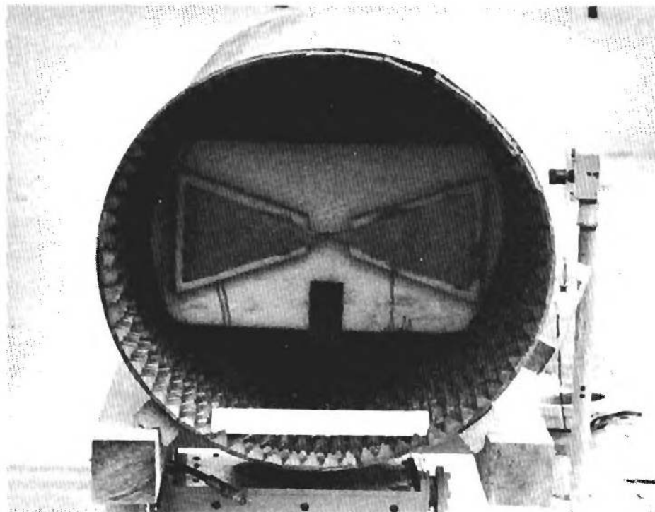
Figure 2. View of the Hooded 18-Inch Bow-Tie Probe Antenna.
