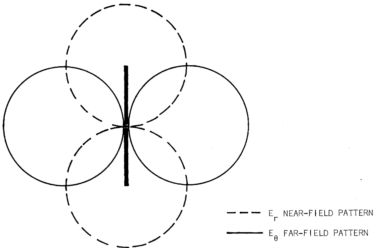
Figure 7: Near-Field and Far-Field Patterns of Short Dipole Antenna.
