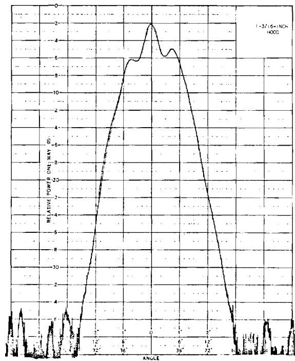
Figure 17. Antenna Patterns for ASN 111A Antenna at 8 GHz.
