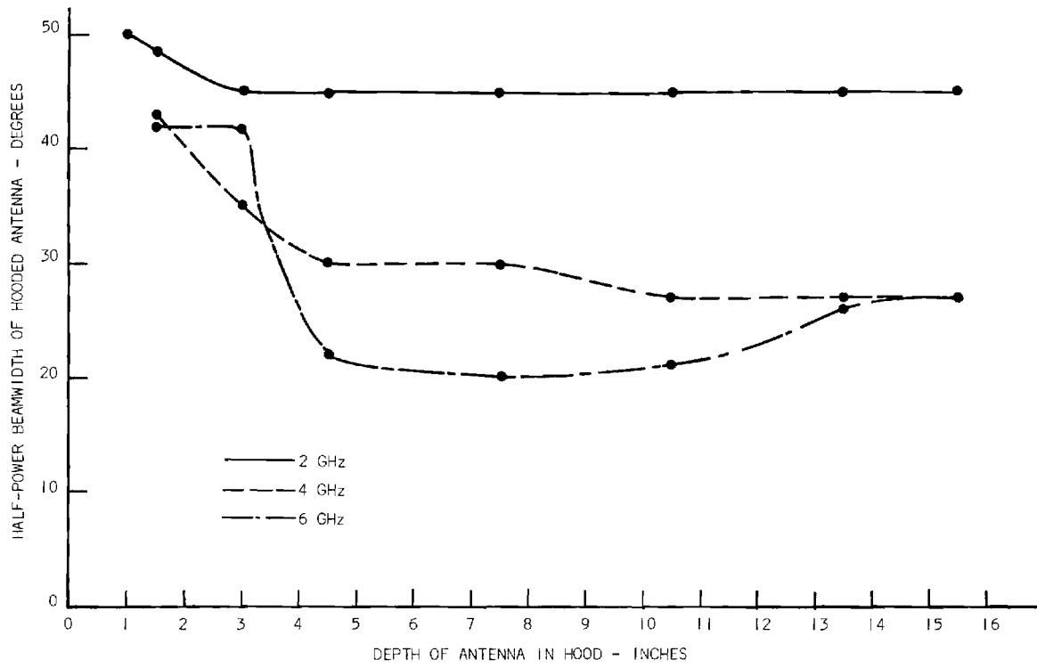
Figure 15. Measured Beamwidth of Hooded Antenna as a Function of Hood Length.
