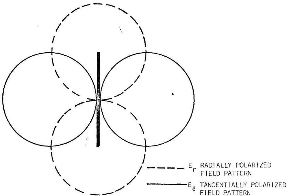
Figure 1. Patterns of the Radially and Tangentially Polarized Electric Field Components of a Short Dipole Antenna.
