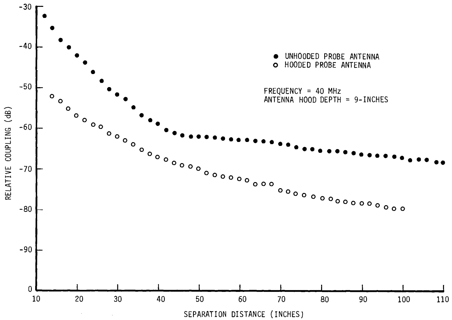
Figure 7. Open-Field Relative Coupling at 40 MHz.
