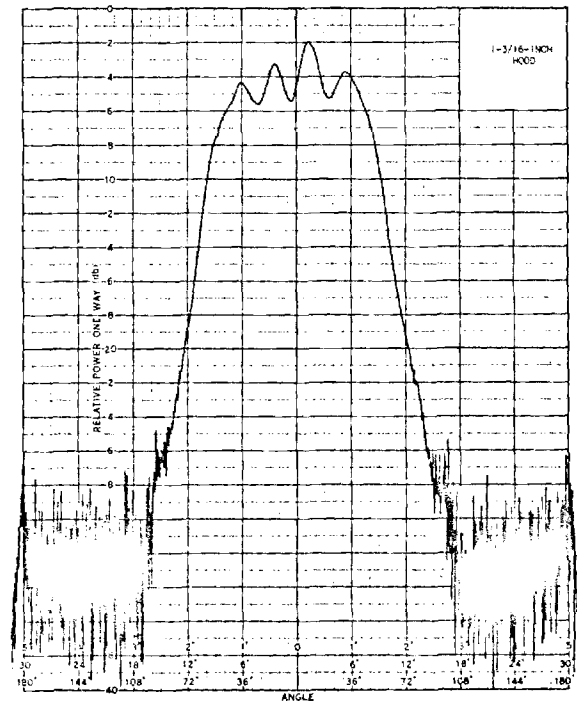
Figure 18. Antenna Patterns for ASN 111A at 10 GHz.
