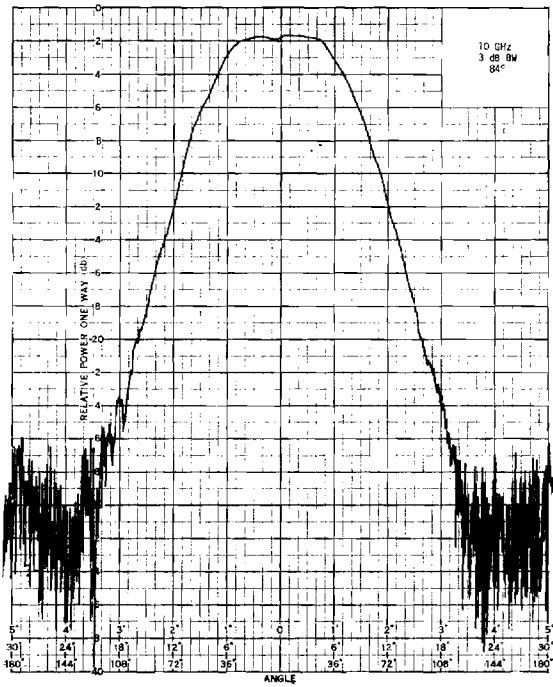
Figure 17. Antenna Patterns for Unhooded ASN 111A Antenna at 4, 6, 8 and 10 GHz.
