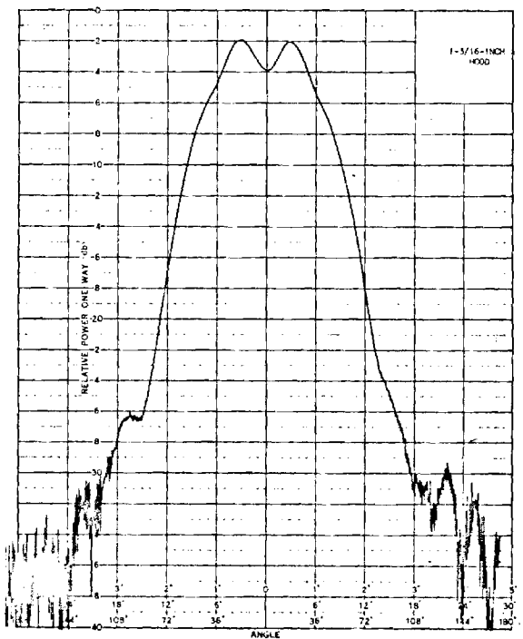
Figure 16. Antenna Patterns for ASN 111A Antenna at 6 GHz.
