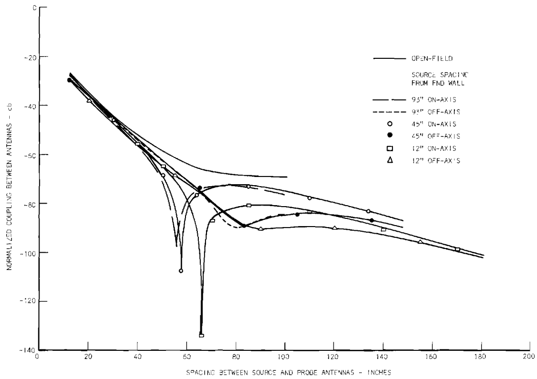
Figure 5. Coupling Between Antennas as a Function of Spacing and Source Location in a Shielded Enclosure at 30 MHz.
