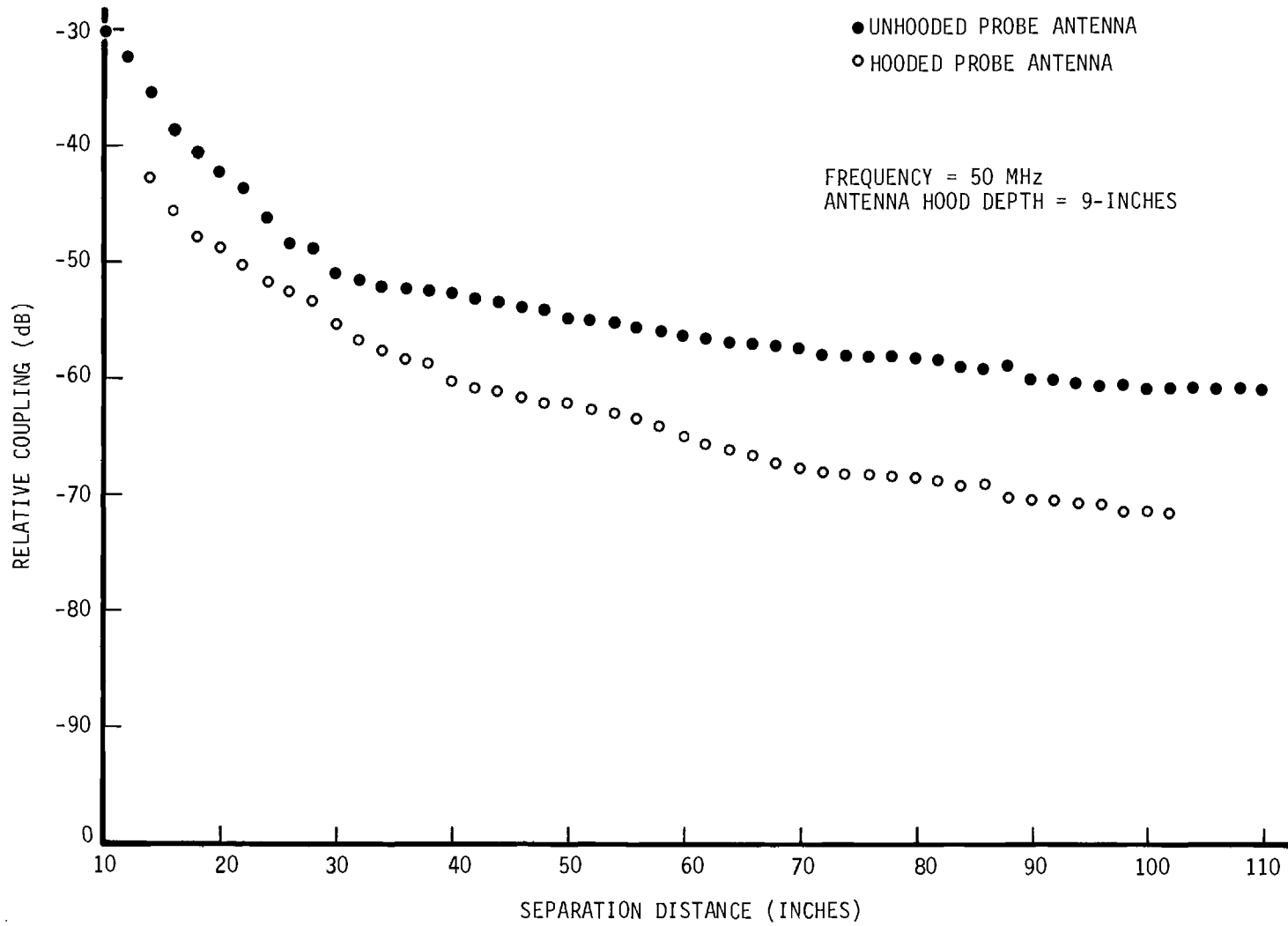
Figure 6. Open-Field Relative Coupling at 50 MHz.
