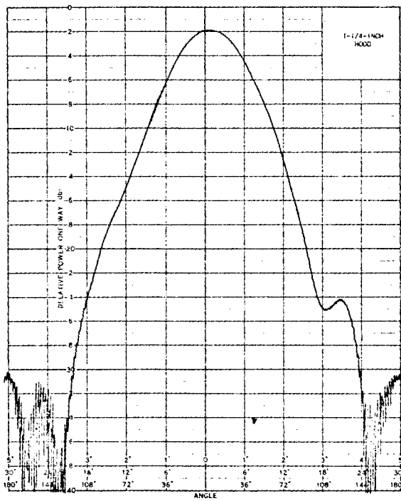
Figure 10. Antenna Patterns for ASN 112A Antenna at 2 GHz.
