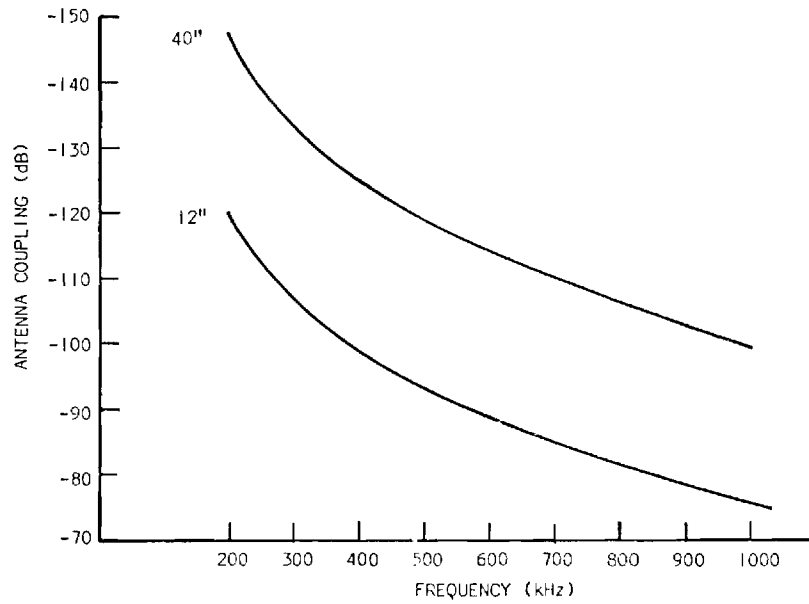
Figure 22. Antenna Coupling as a Function of Frequency for Two 30-Inch Bow-Tie Antennas in a Shielded Enclosure.
