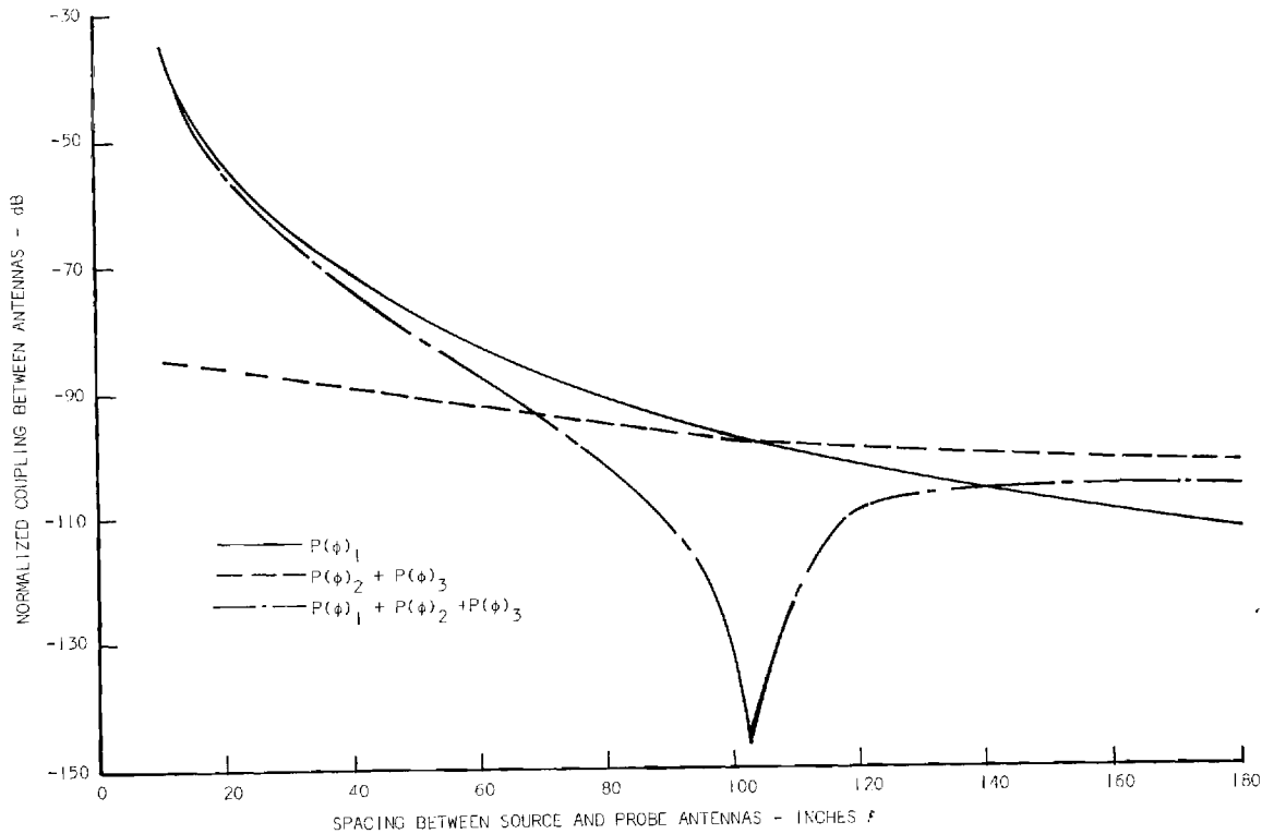
Figure 9. Diagram of Theoretical Coupling Null in a Shielded Enclosure.
