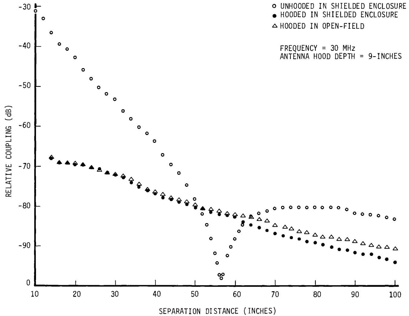
Figure 5. Relative Coupling as a Function of Antenna Separation Distance at a Frequency of 30 MHz.
