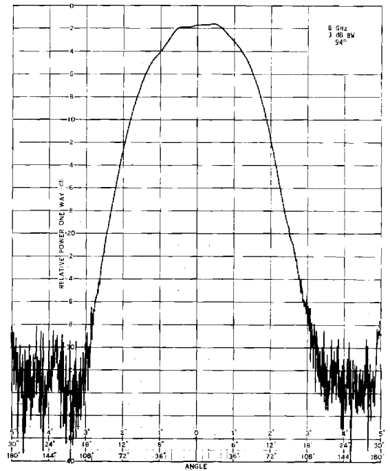
Figure 13. Antenna Patterns for Unhooded ASN 116A Antenna at 2, 3, 4 and 6 GHz.
