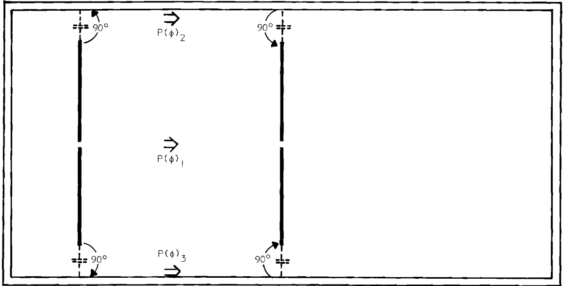
Figure 8. Diagram Showing Three Primary Coupling Paths Between Two Dipole Antennas in a Shielded Enclosure at Low Frequencies.
