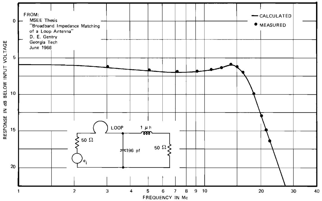
Figure 67. Response of a Three Element Chebyshev Lowpass Filter with a 1 dB Ripple ( R_s = 50 ohms).
