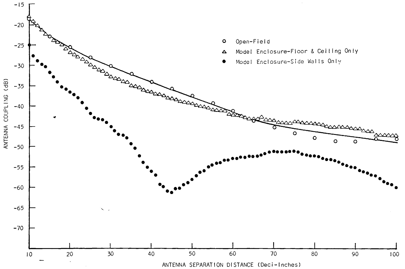
Figure 5. Coupling Between Two Horizontal Bow-Tie Antennas in a Model Enclosure as a Function of Separation at 400 MHz.
