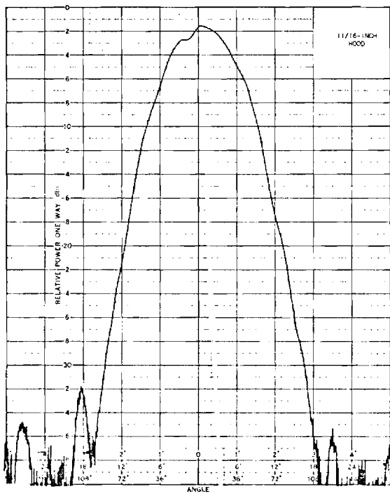
Figure 17. Antenna Patterns for ASN 111A Antenna at 8 GHz.
