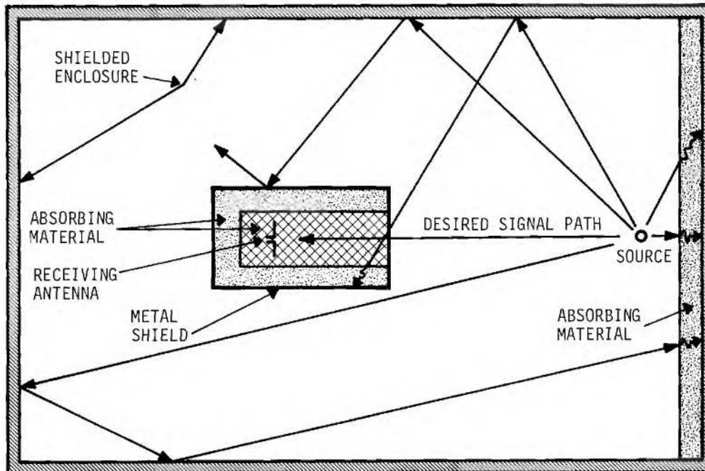
Figure 3. Diagram of a Hooded Antenna Measurement Setup in a Shielded Enclosure.
