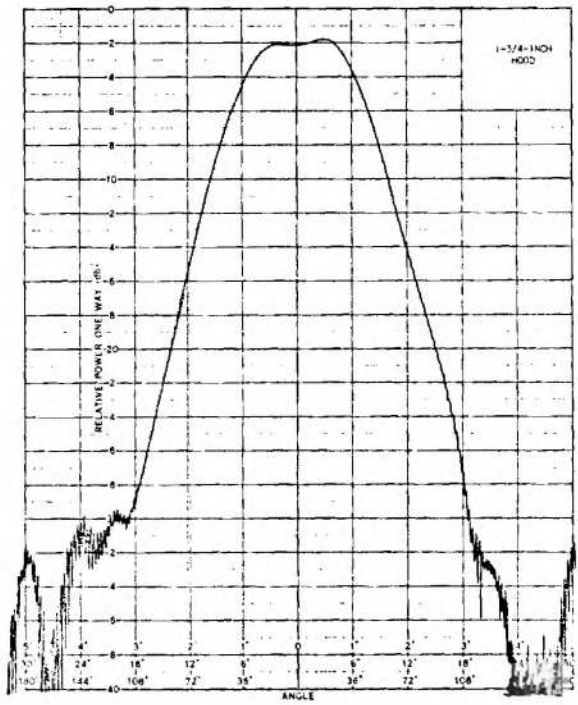
Figure 11. Antenna Patterns for ASN 112A Antenna at 3 GHz.
