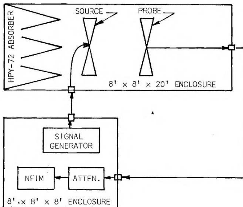
Figure 19. Block Diagram of Low Frequency Coupling Measurement Configuration.
