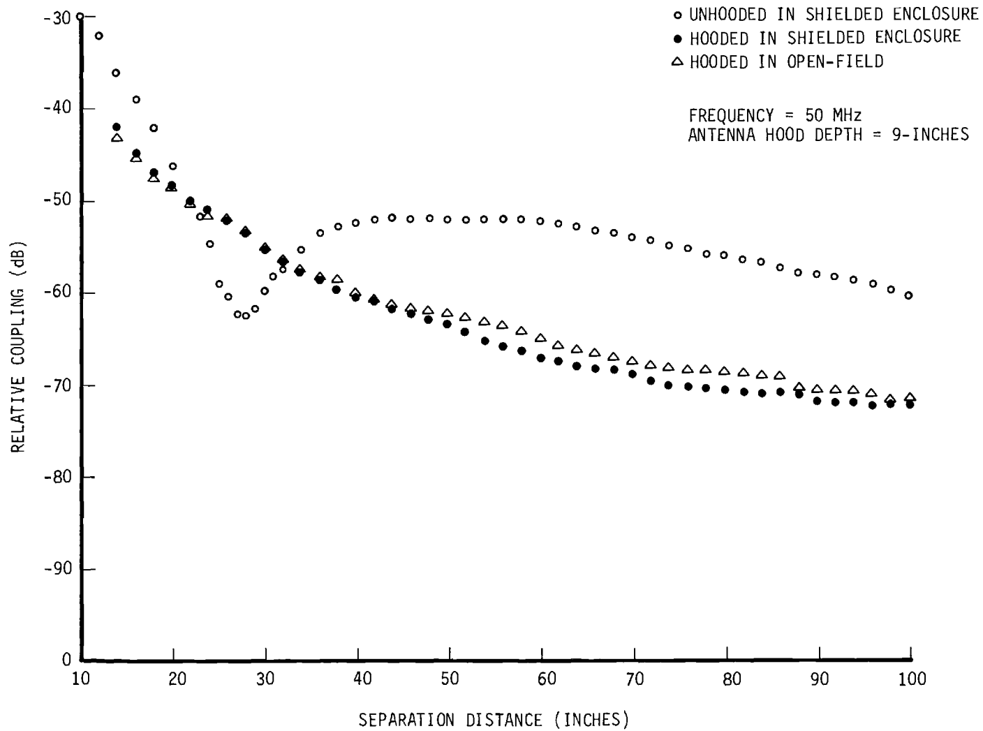
Figure 3. Relative Coupling as a Function of Antenna Separation Distance at a Frequency of 50 MHz.
