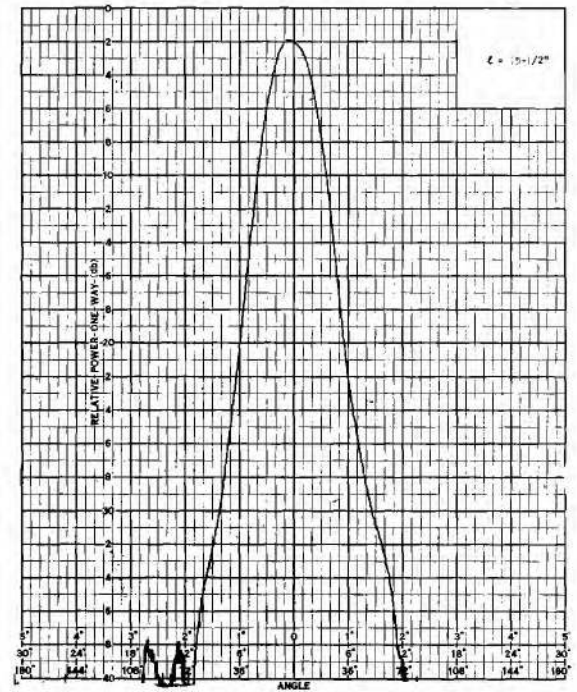
Figure 13. Patterns of Hooded Antenna as a Function of Hood Length at 4 GHz.
