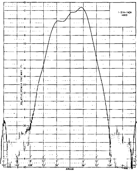
Figure 12. Antenna Patterns for ASN 112A Antenna at 4 GHz.
