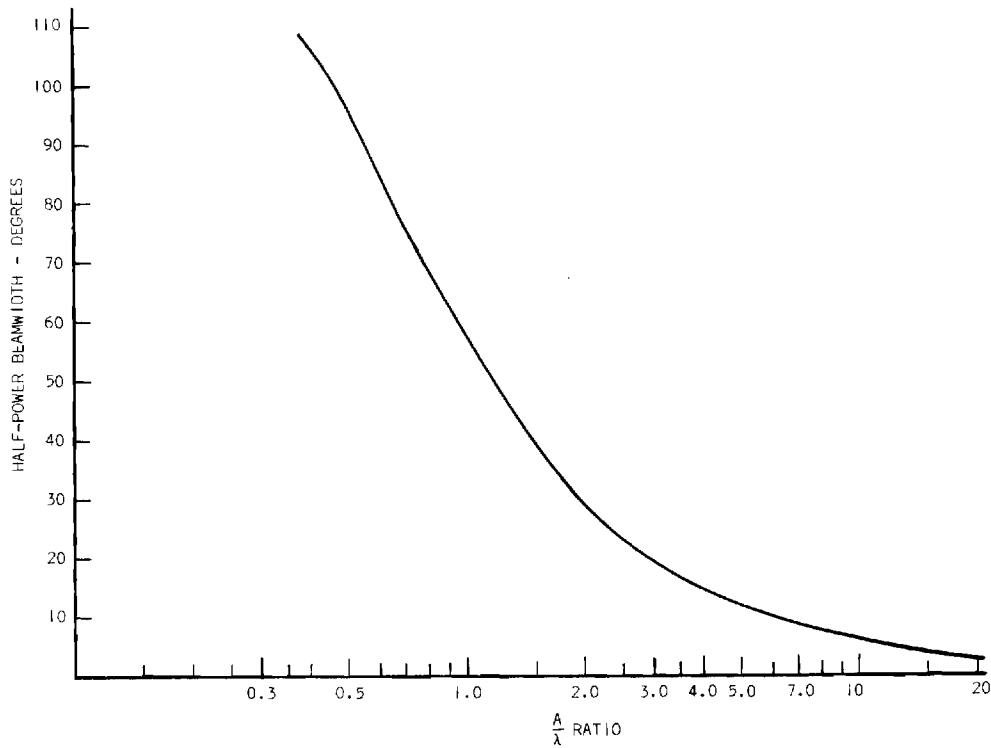
Figure 10. Theoretical Beamwidth of Hooded Antenna Vs. Aperture Size.
