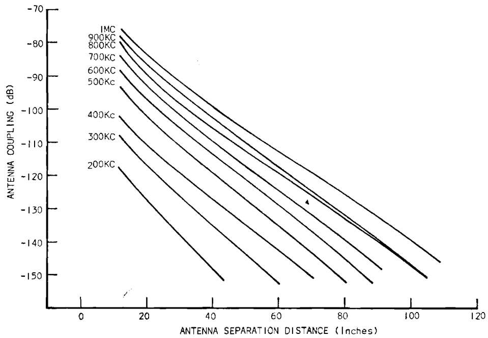
Figure 21. Antenna Coupling as a Function of Separation Distance for Two 30-Inch Bow-Tie Antennas in a Shielded Enclosure.
