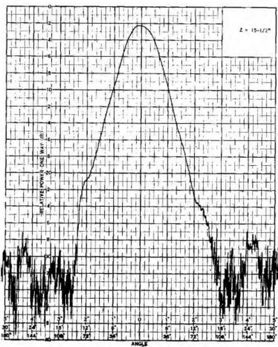
Figure 12. Patterns of Hooded Antenna as a Function of Hood Length at 2 GHz.
