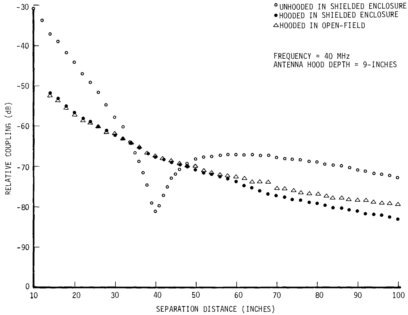
Figure 4. Relative Coupling as a Function of Antenna Separation Distance at a Frequency of 40 MHz.
