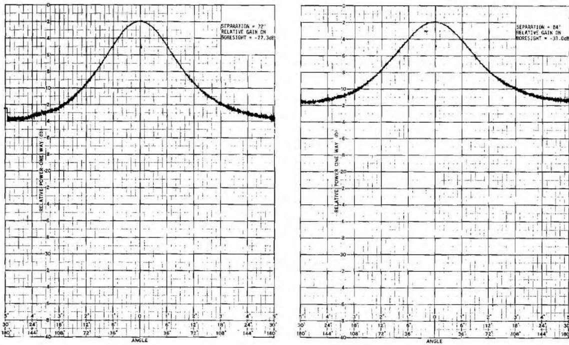
Figure 11. Near-Field Mutual Coupling Between a Dipole and Hooded Probe Antenna at Separation Distances of 72 and 84 Inches.
