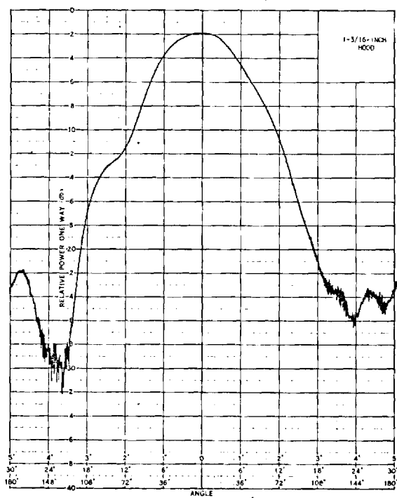
Figure 14. Antenna Patterns for AEL Model ASN 111A Cavity-Backed Spiral Antenna at 2 GHz.
