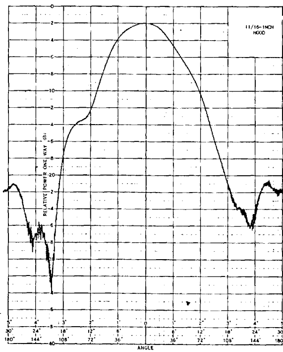
Figure 14. Antenna Patterns for AEL Model ASN 111A Cavity-Backed Spiral Antenna at 2 GHz.
