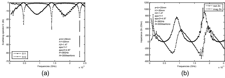
Figure 9. (a) The diffraction operator S; (b) The impedance Zin as a fuction of frequency
