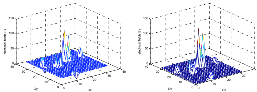
Figure 7. The electrical fields to the sub domains: metal, dielectric, source and transistor.
