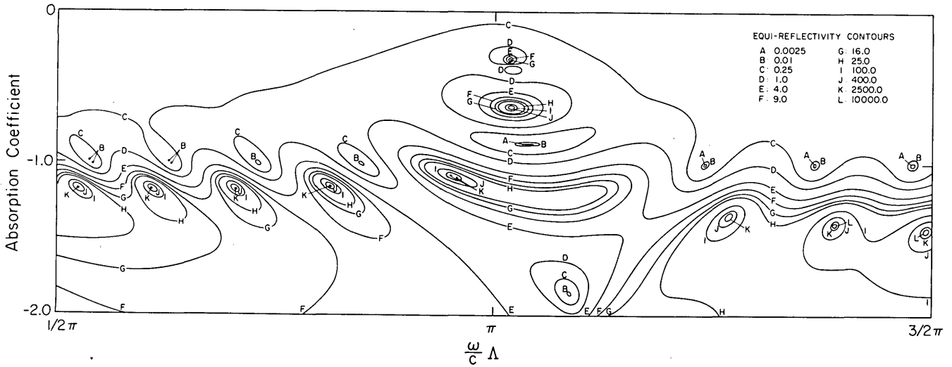
FIG. 6. Contours of equal reflectivity in \omega-\alpha_2 plane.
