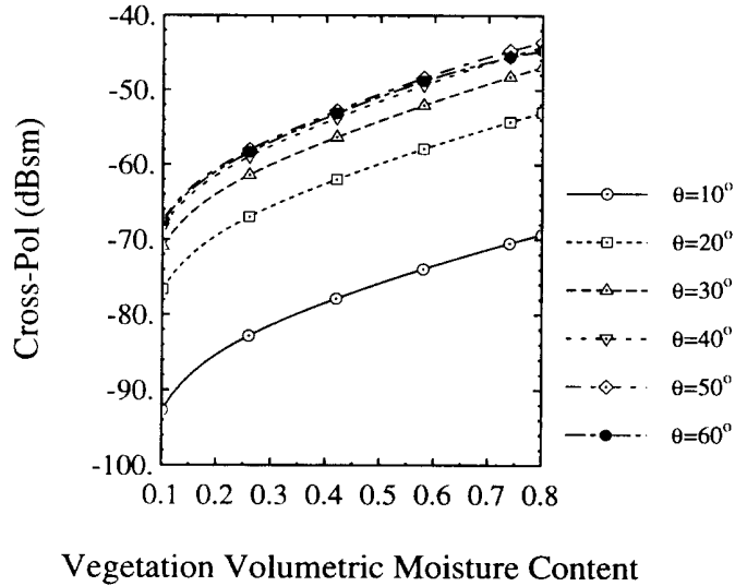
Figure 13: The cross-polarized RCS of the cylinder-rough surface composite target versus the volumetric moisture content of the vertical cylinder ( a = 0.385\text{m} , l_c = 0.71\text{m} , ks = 0.1 , kl = 3.0 , and \epsilon_g = 4.9 + i0.9 ).
