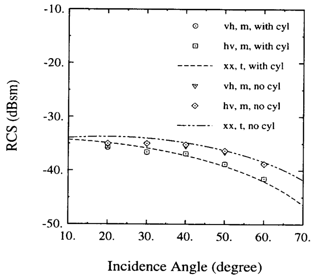
Figure 17: The cross-polarized RCS of a water cylinder with a = 0.83\text{cm} and l_c = 11.0\text{cm} above the rough surface at 9.25 GHz. The RCS of the rough surface alone ( \sigma_{pq}^0 A ) is also shown for comparison.
