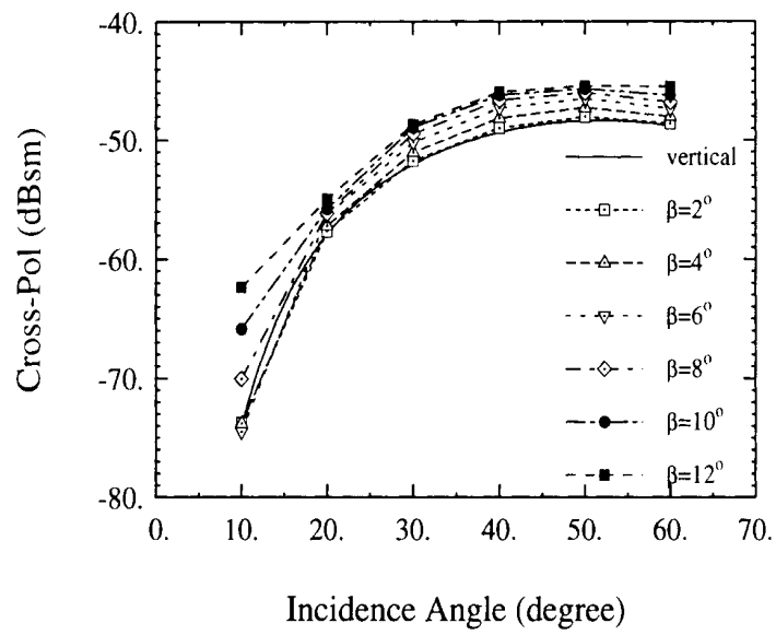
Figure 7: The cross-polarized RCS caused by the interaction between a cylinder ( a = 0.385\text{cm} , l_c = 0.71\text{m} , and \epsilon_c = 43.4 + i13.2 ) and a rough surface ( ks = 0.1 , kl = 3.0 , and \epsilon_g = 4.9 + i0.9 ).
