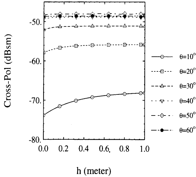
Figure 12: The cross-polarized RCS of the cylinder-rough surface composite target versus the height of the cylinder lower end above the ground ( a = 0.385\text{m} , l_c = 0.71\text{m} , \epsilon_c = 43.4 + i13.2 , ks = 0.1 , kl = 3.0 , and \epsilon_g = 4.9 + i0.9 ).
