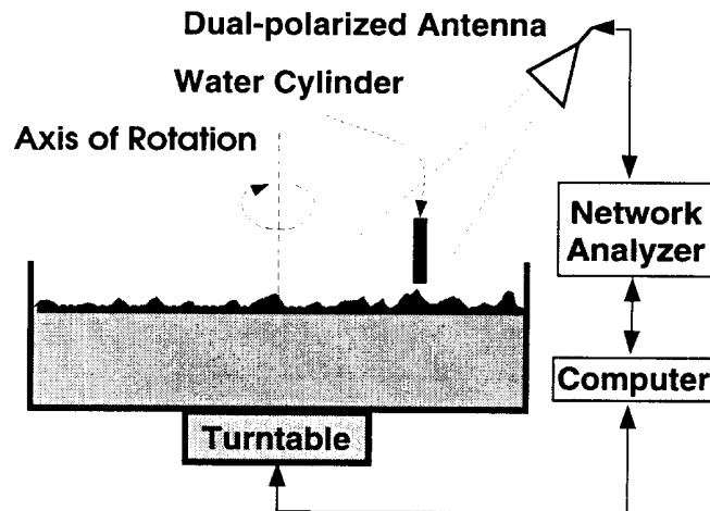
Figure 15: The experimental setup for the backscatter measurement of a vertical cylinder above a rough ground plane.
