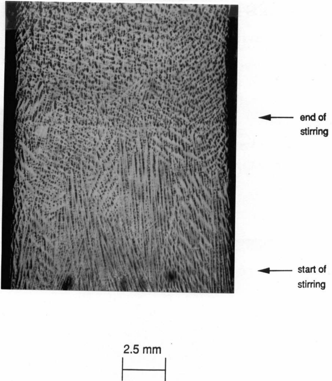
Figure 4.52: Microphotograph of sample 4 in fig. 3.18.
