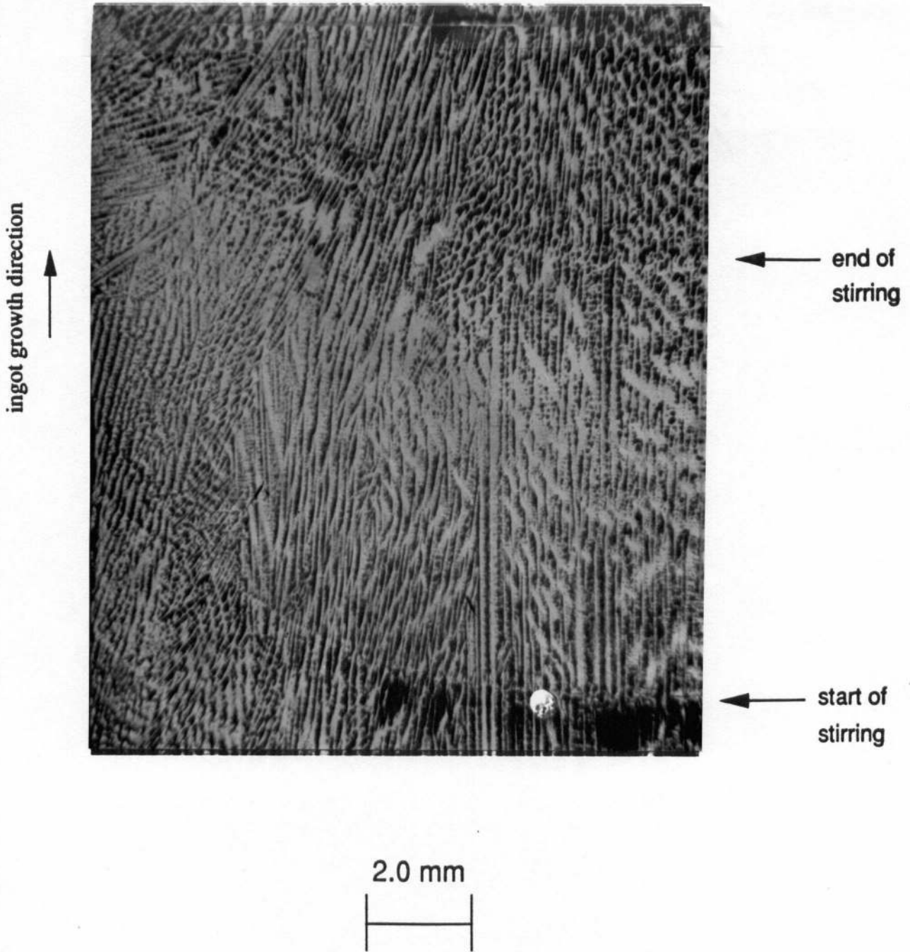
Figure 4.49: Microphotograph of sample 1 in fig. 3.18.
