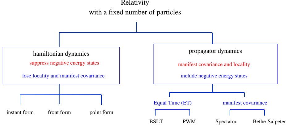
Fig. 5. Classification of relativistic methods. The class on the right is propagator dynamics ( \mathcal{P} ) and on the left is hamiltonian dynamics ( \mathcal{H} ).
