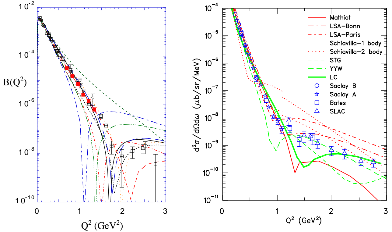
Fig. 8. Theory and data for the elastic B structure function (left panel) and the threshold electrodisintegration cross section (right panel). The calculations listed in Table 1 are shown in the left panel.
