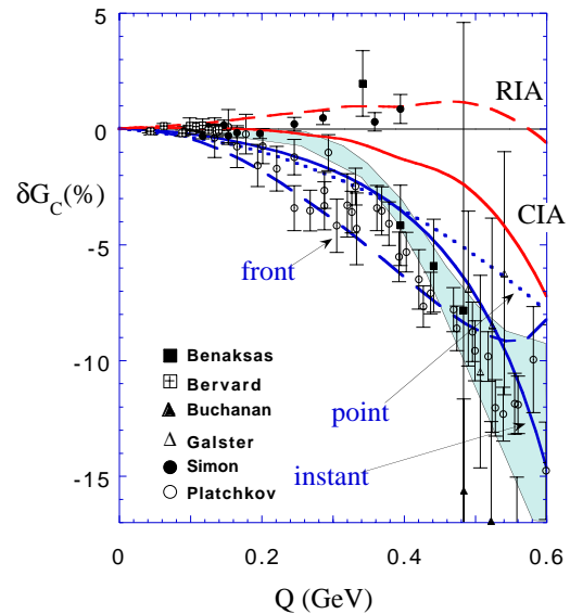
Fig. 6. Comparison of selected relativistic calculations of G_C with charge form factor data. The shaded area is the best fit (with errors) determined by Sick [2]. All curves and data are expressed as a percentage difference from the AV18 calculation in NRIA.
