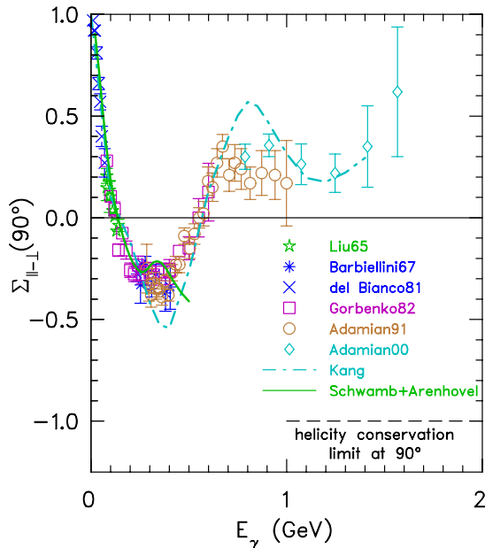
Fig. 10. Polarized photon asymmetry \Sigma at \theta_{cm} = 90^\circ . For discussion and references see Ref. [3].
