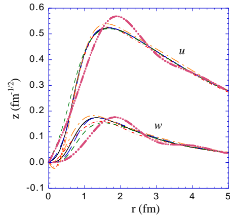
Fig. 1. The u and w wavefunctions in r space for six models discussed in the text.
