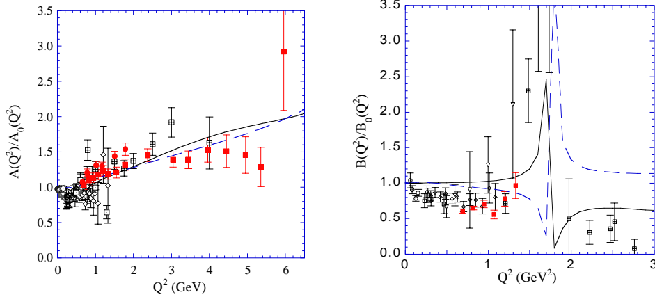
Fig. 7. Ratios of the structure functions A and B with different choices for the form factors F_3 or f_{\rho\pi\gamma} normalized to A_0 and B_0 calculated with the “standard” choices F_3 =dipole and f_{\rho\pi\gamma} = 0 . Solid line: F_3 =tripole, f_{\rho\pi\gamma} = 0 . Dashed line: F_3 =dipole, f_{\rho\pi\gamma} =dipole with \Lambda_d^2=1.5 \text{ GeV}^2 .
