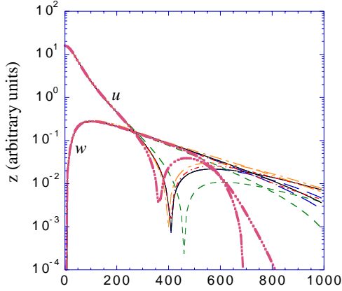
Fig. 2. The u and w wavefunctions in p space for six models discussed in the text. (Each model is normalized so that u(0) = 16 .)
